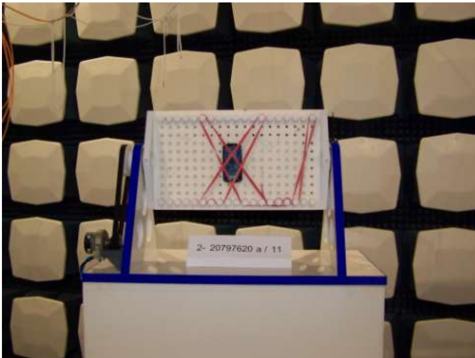
Radiated measurements in anechoic chamber
