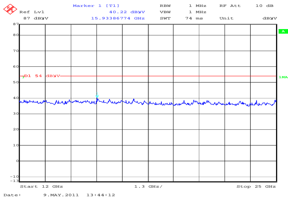
Plot 4: Receiver mode (12 GHz – 25 GHz) (horizontal / vertical – max hold)
