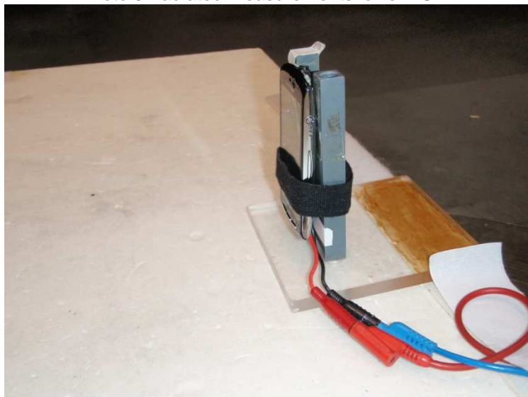
Photo 5: radiated measurements lower 1GHz
