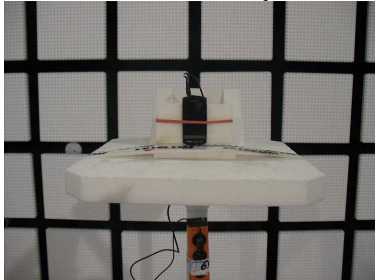
Photo 2: radiated measurements higher 1GHz
