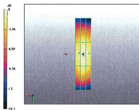
0 dB = 0.493A/m
