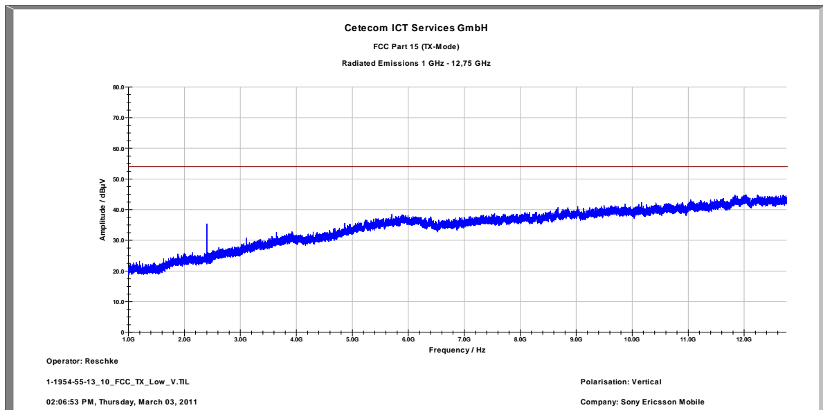
Plot 2: 1 GHz to 12.75 GHz, vertical polarization
