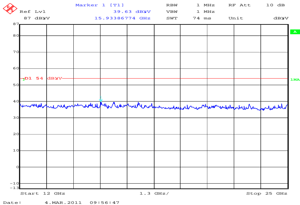
Plot 4: 12 GHz to 25 GHz
