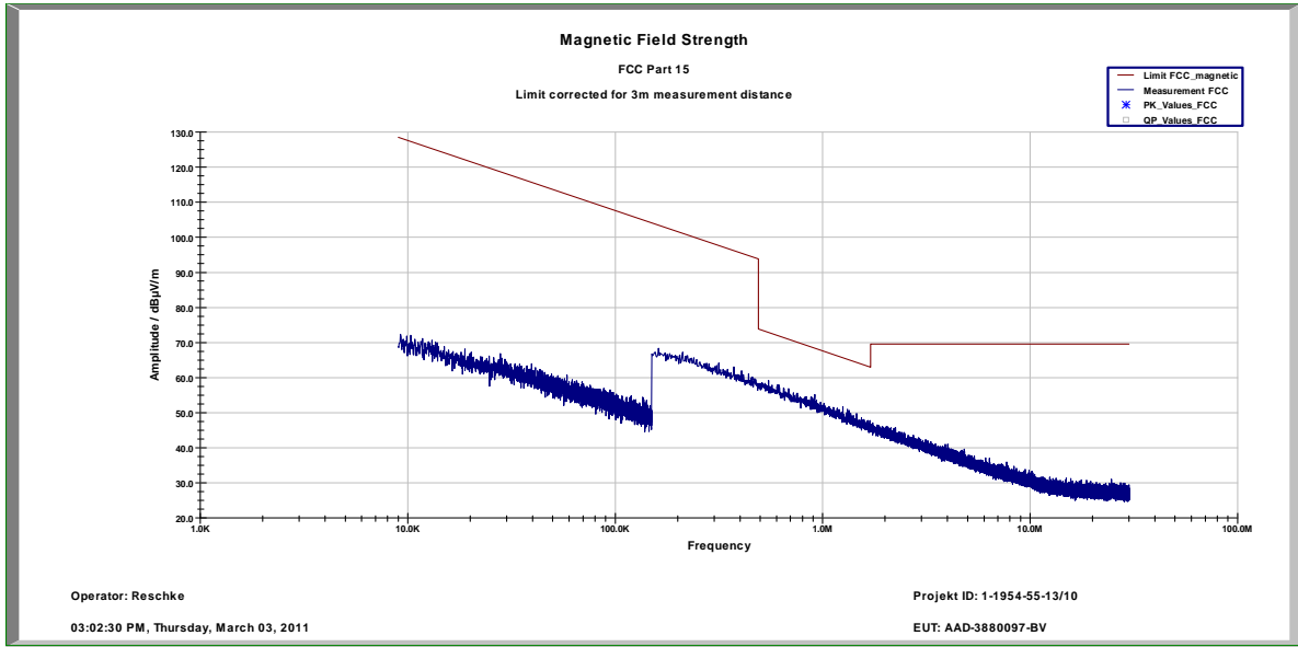
Plot 1: 9 kHz to 30 MHz / channel 39 (valid for all channels)
