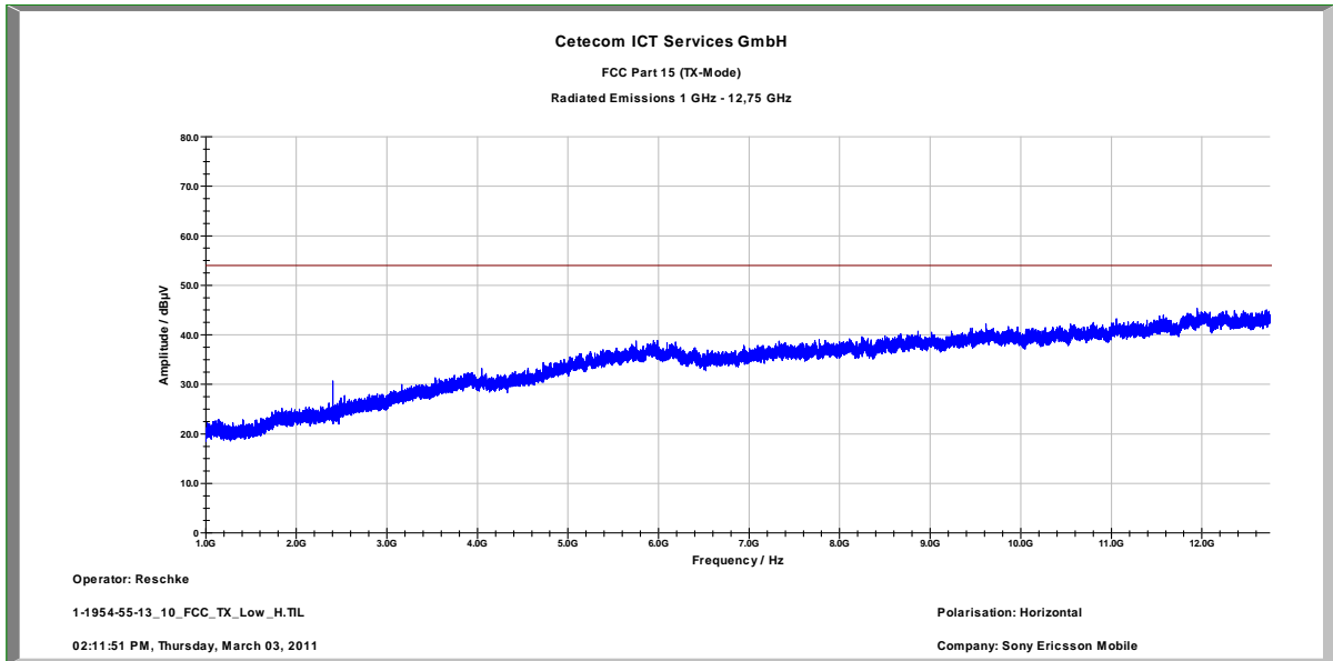
Plot 3: Lowest channel, 1 GHz to 12.75 GHz, horizontal polarization
