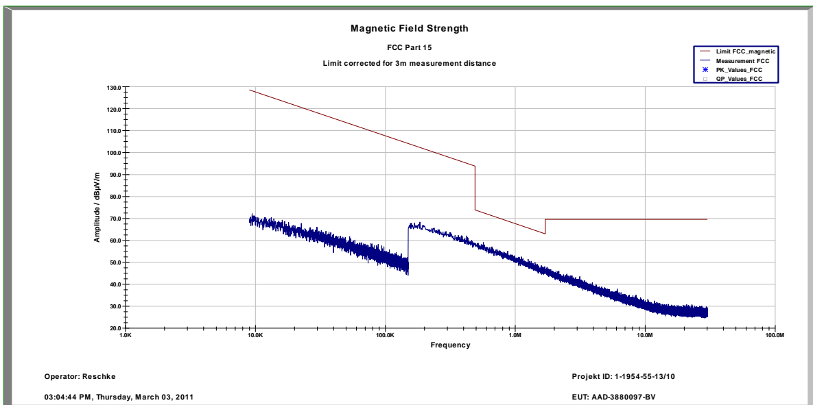
Plot 1: 9 kHz to 30 MHz
