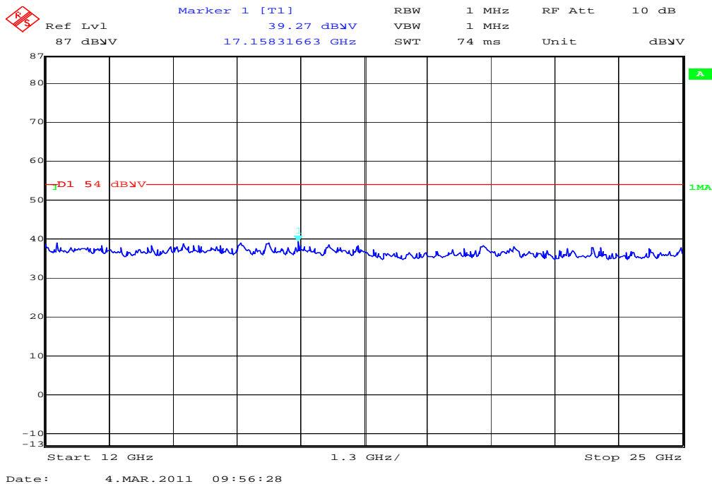
Plot 4: Lowest channel, 12 GHz to 25 GHz (valid for all channels)
