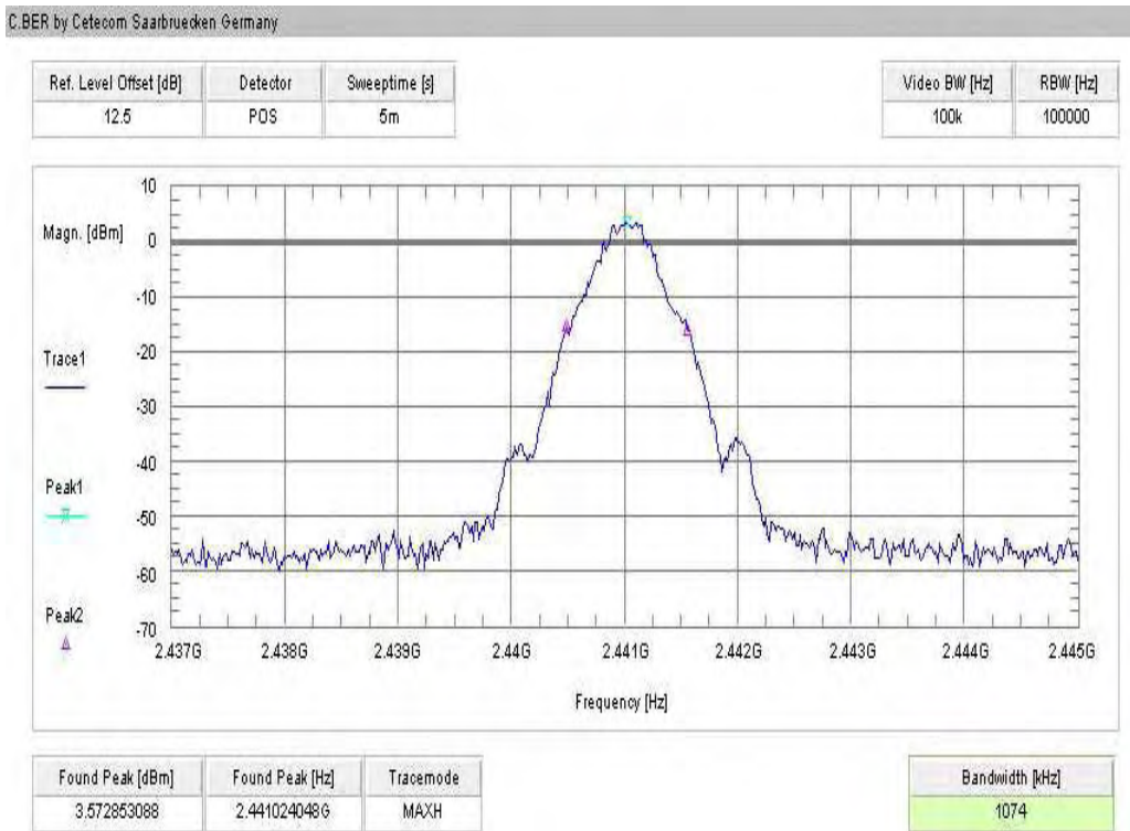
Plot 2: TX mode, channel 39, 20 dB bandwidth
