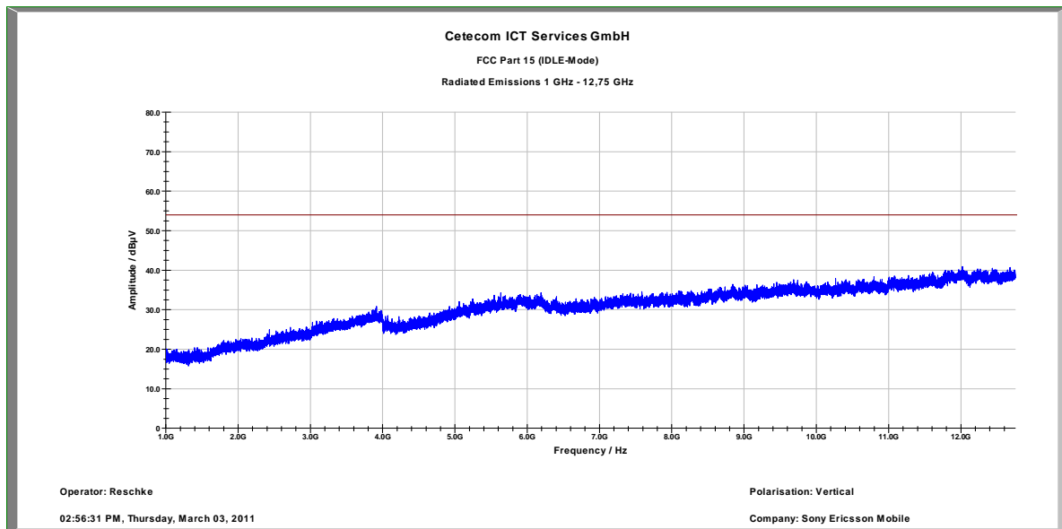
Plot 2: 1 GHz to 12.75 GHz, vertical polarization
