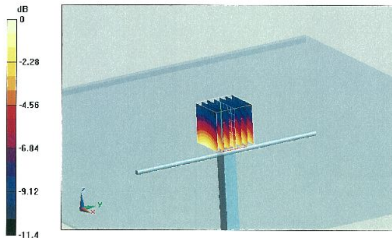
0 dB = 3.27mW/g
