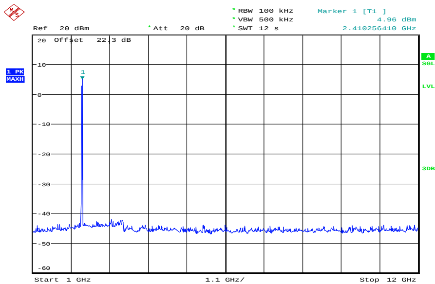
Plot 2: TX mode, lowest channel, 1 GHz to 12 GHz
