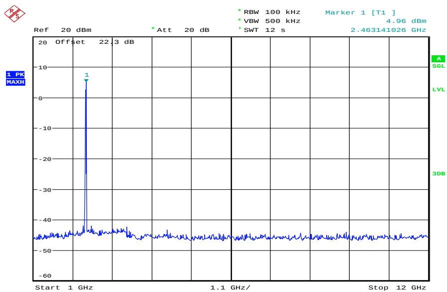
Plot 8: TX mode, highest channel, 1 GHz to 12 GHz
