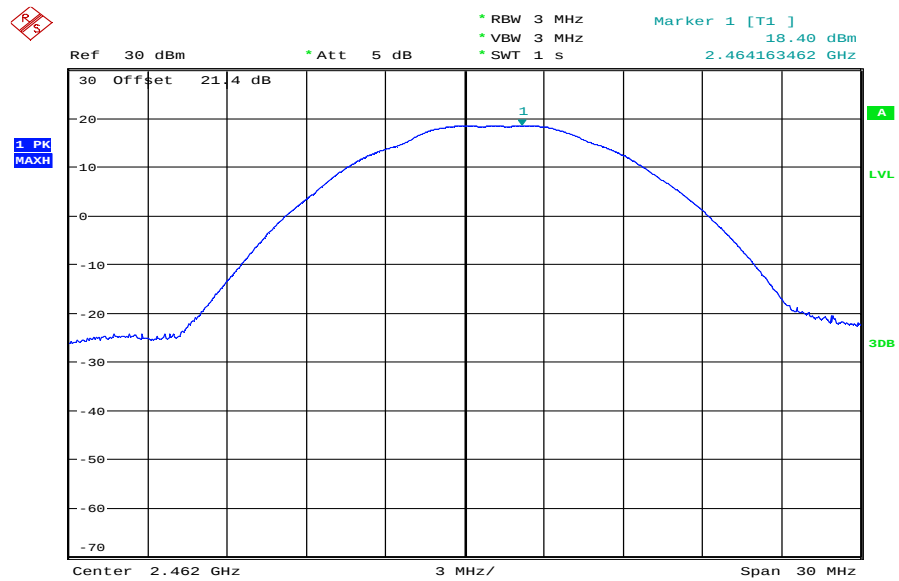
Plot 3: TX mode, highest channel, 5.5 MBit/s
