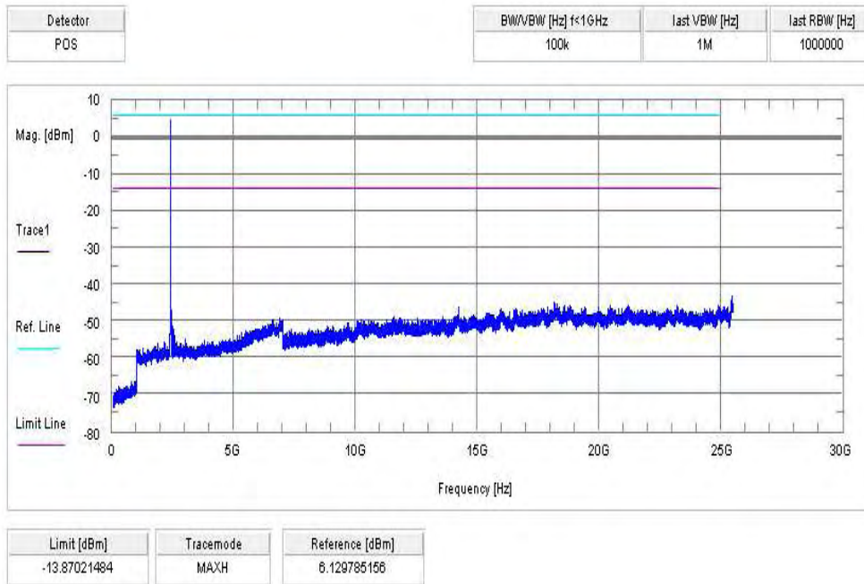
Plot 7: lowest channel, 8 DPSK modulation
