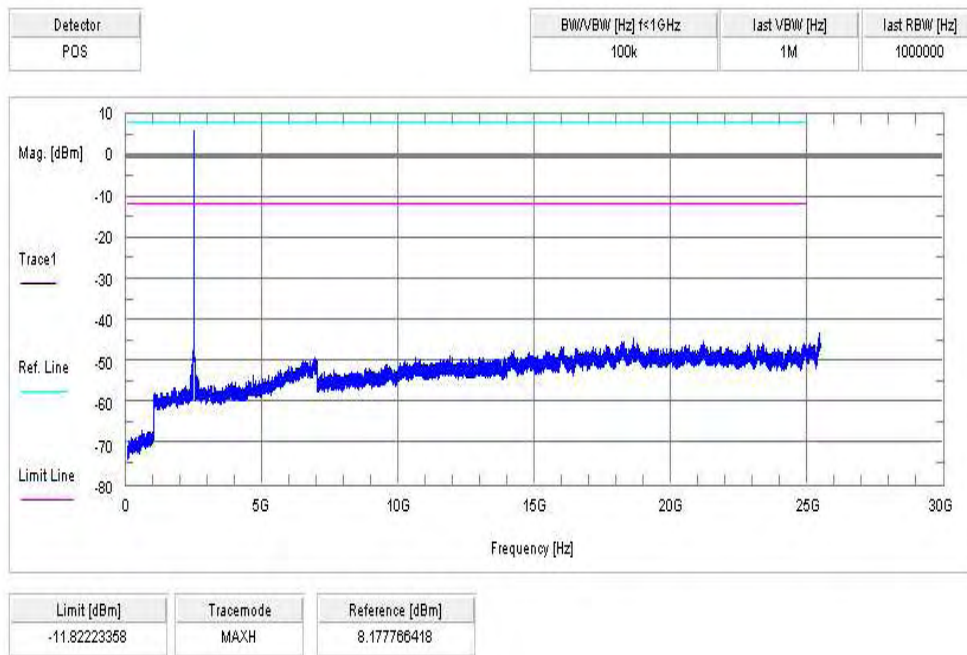
Plot 9: highest channel, 8 DPSK modulation
