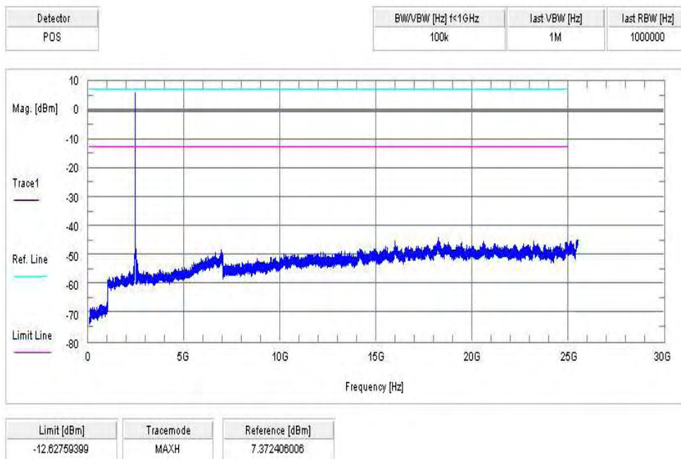
Plot 2: middle channel, GFSK modulation
