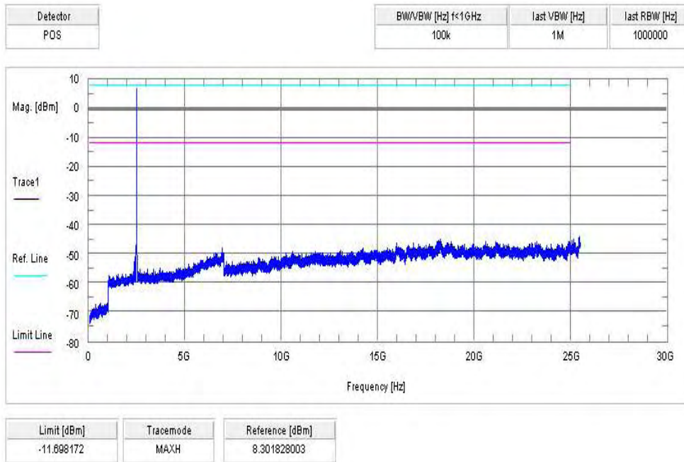
Plot 3: highest channel, GFSK modulation
