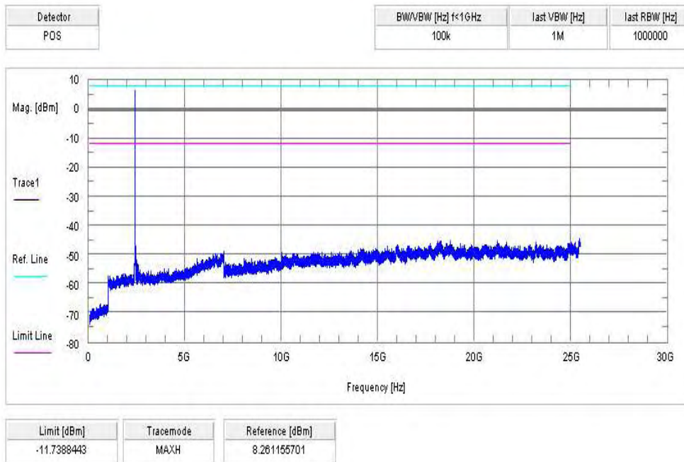
Plot 4: lowest channel, Pi/4 DQPSK modulation
