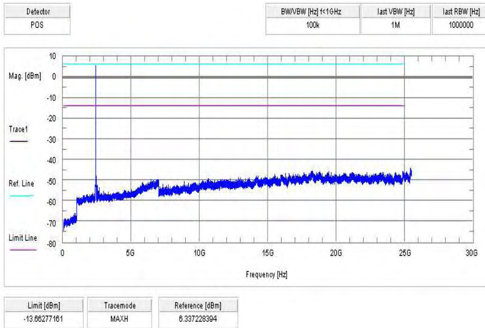
Plot 1: lowest channel, GFSK modulation
