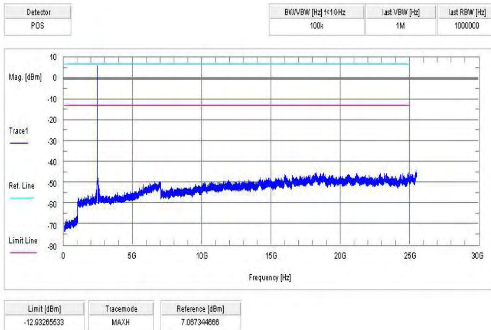
Plot 8: middle channel, 8 DPSK modulation
