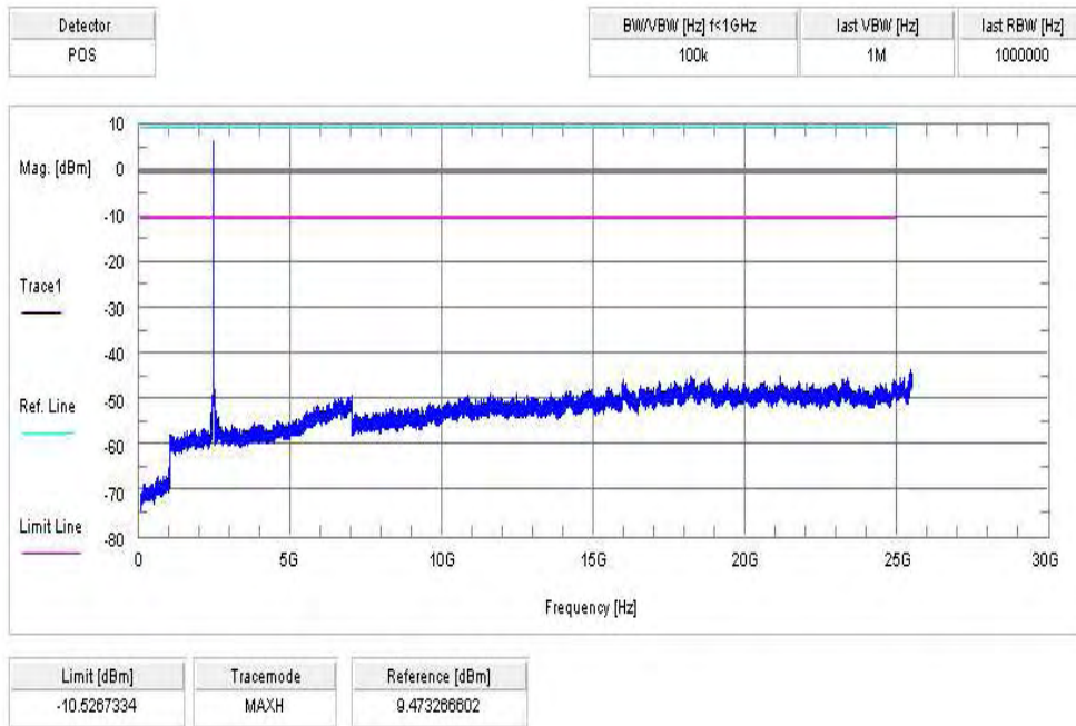
Plot 5: middle channel, Pi/4 DQPSK modulation
