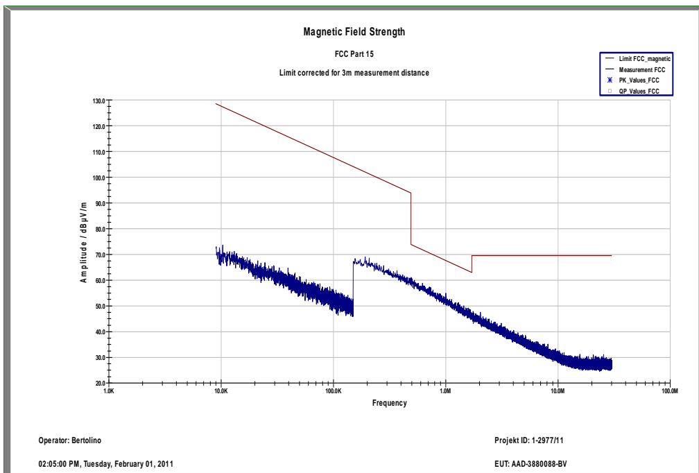
Plot 4: idle / RX – mode, 9 kHz to 30 MHz
