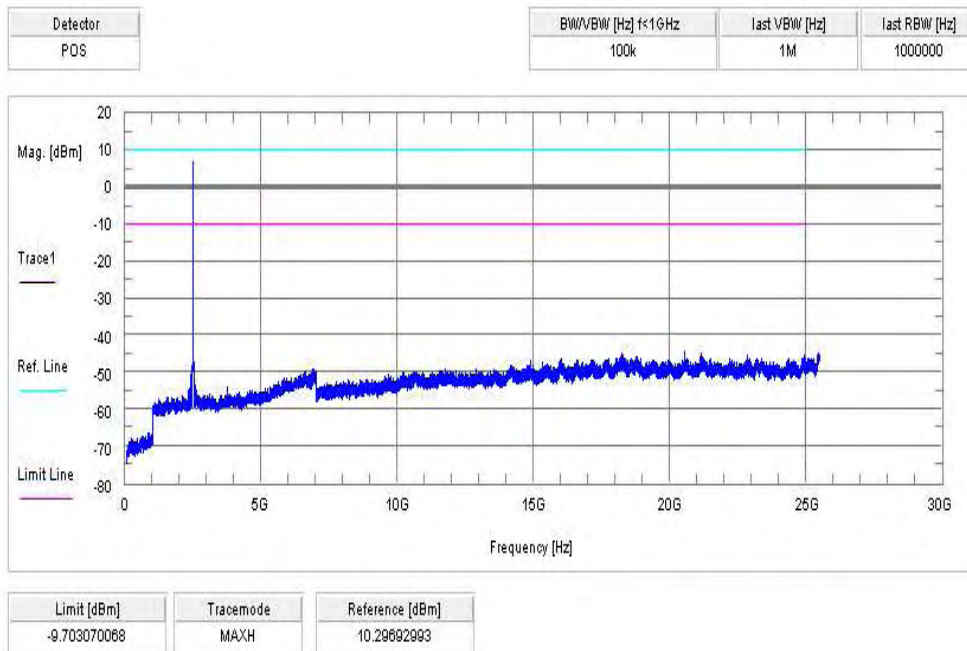
Plot 6: highest channel, Pi/4 DQPSK modulation
