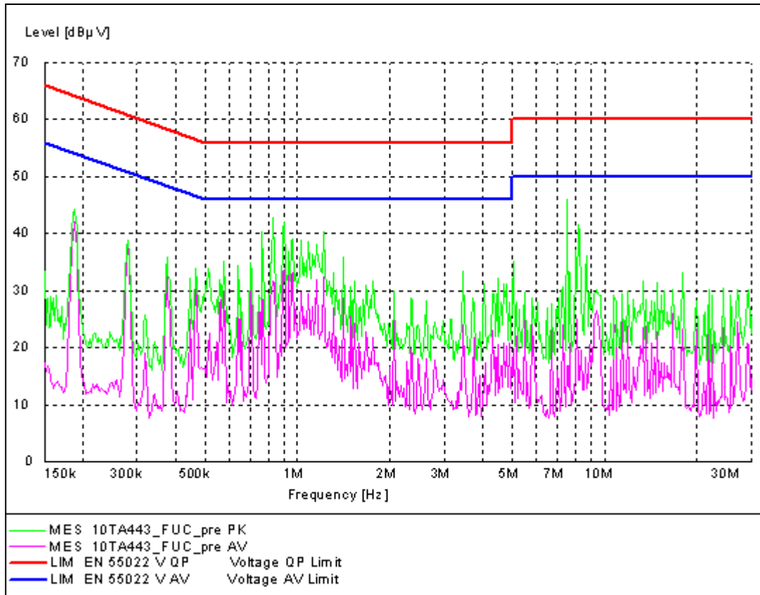
Fig B.3 Conducted Continuous Emission from 150 kHz to 30 MHz
