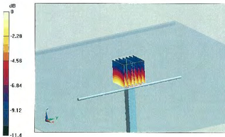
0 dB = 3.27mW/g
