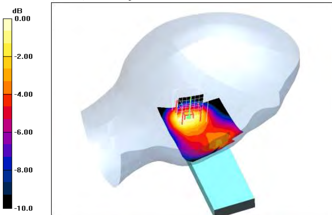
0 dB = 0.164mW/g
