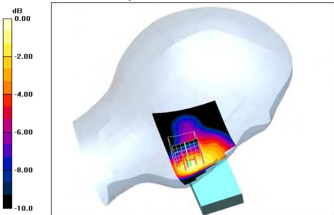
0 dB = 0.403mW/g
