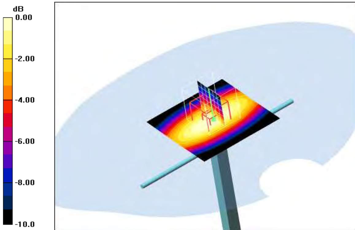
0 dB = 11.9mW/g
