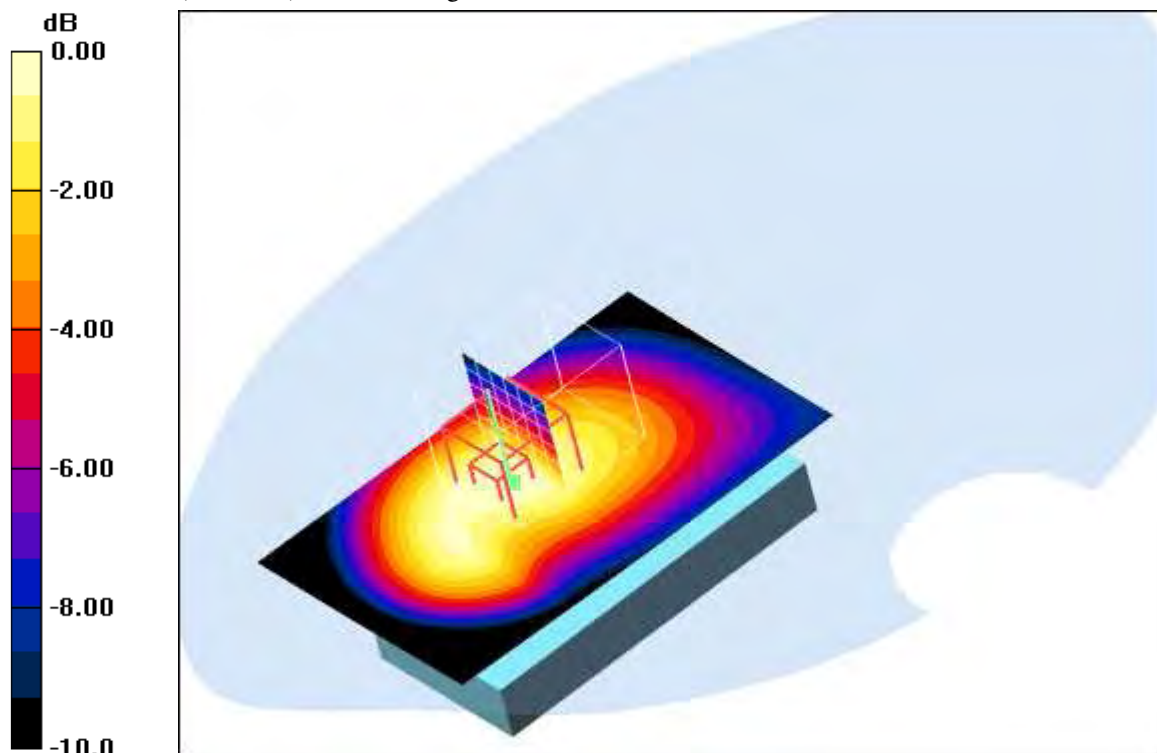
0 dB = 0.356mW/g
