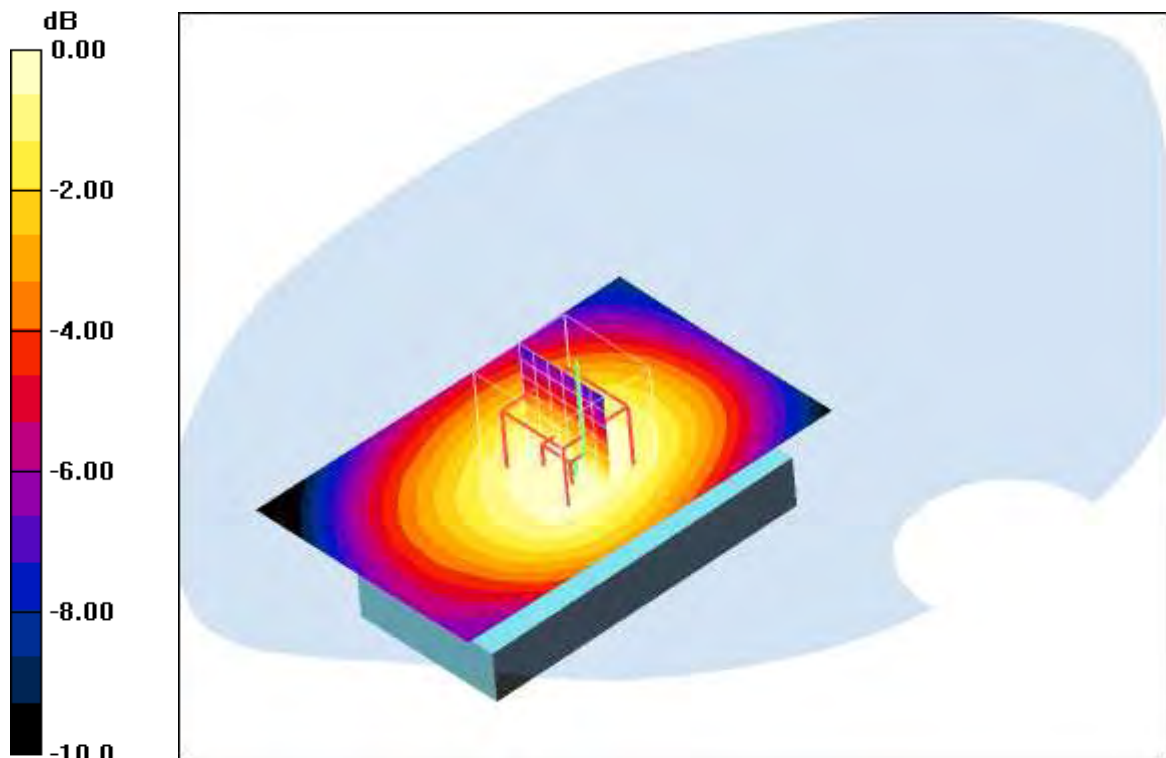
0 dB = 0.130mW/g
