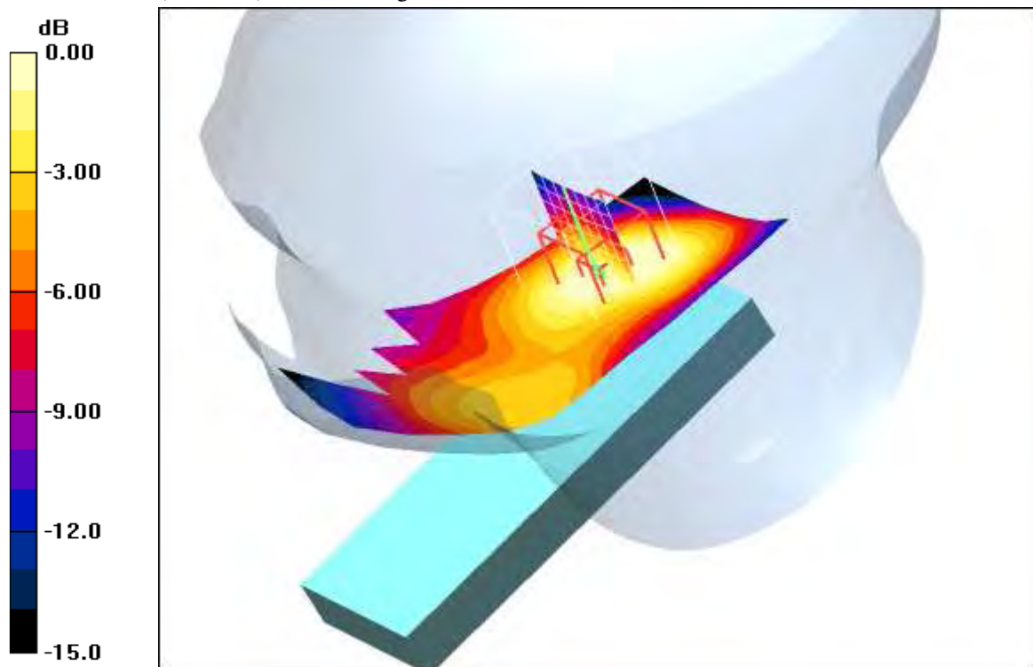
0 dB = 0.151mW/g
