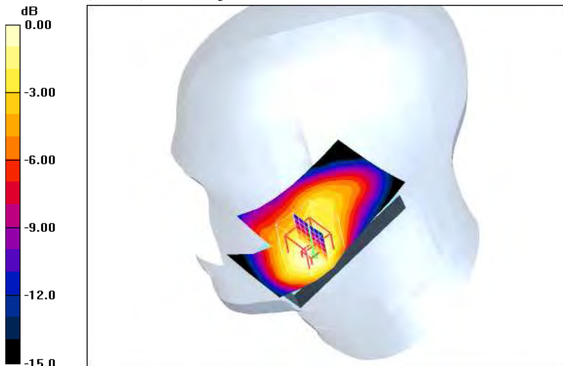
0 dB = 0.537mW/g
