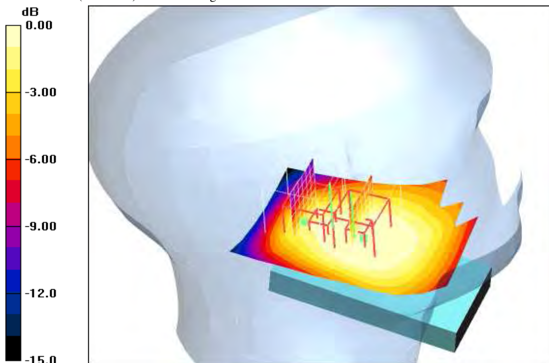
0 dB = 0.157mW/g
