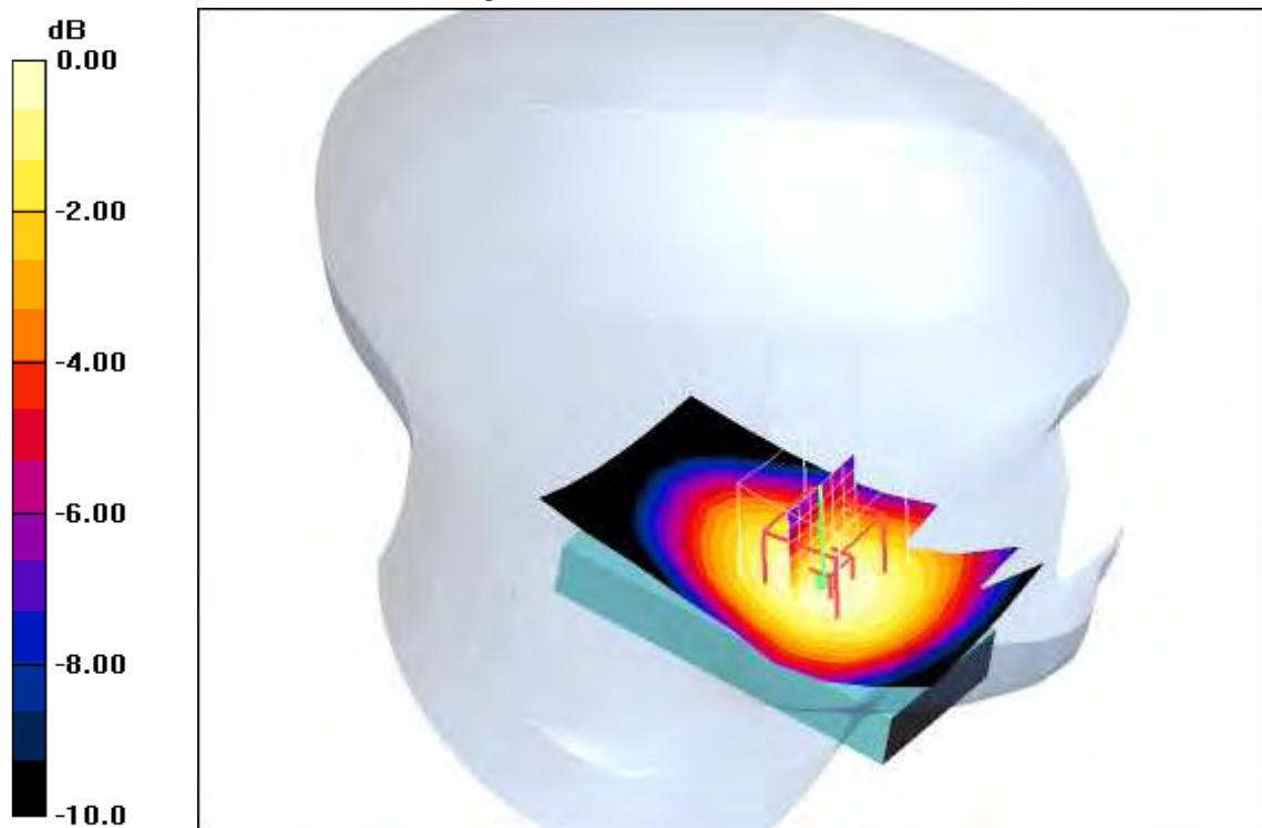
0 dB = 0.281mW/g
