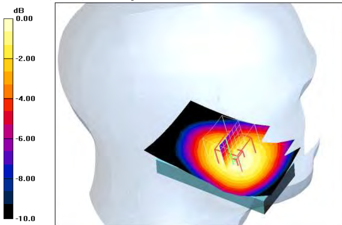
0 dB = 0.406mW/g
