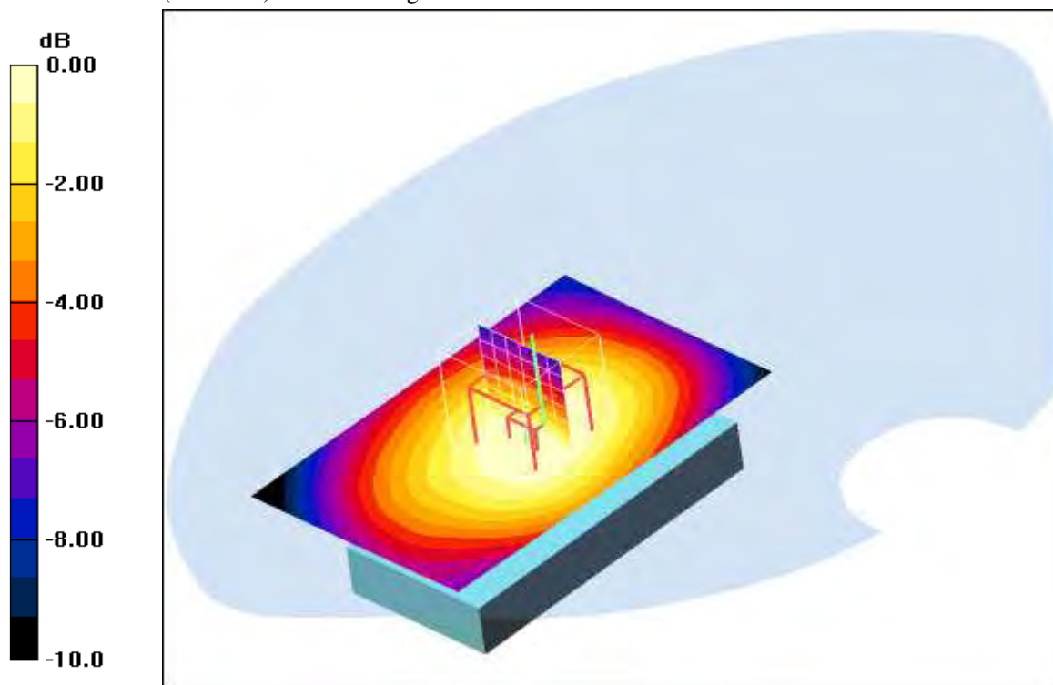
0 dB = 0.204mW/g
