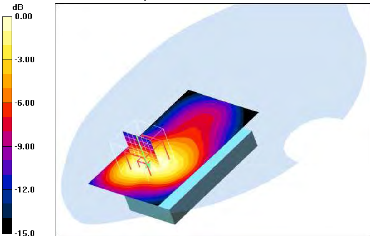
0 dB = 0.408mW/g
