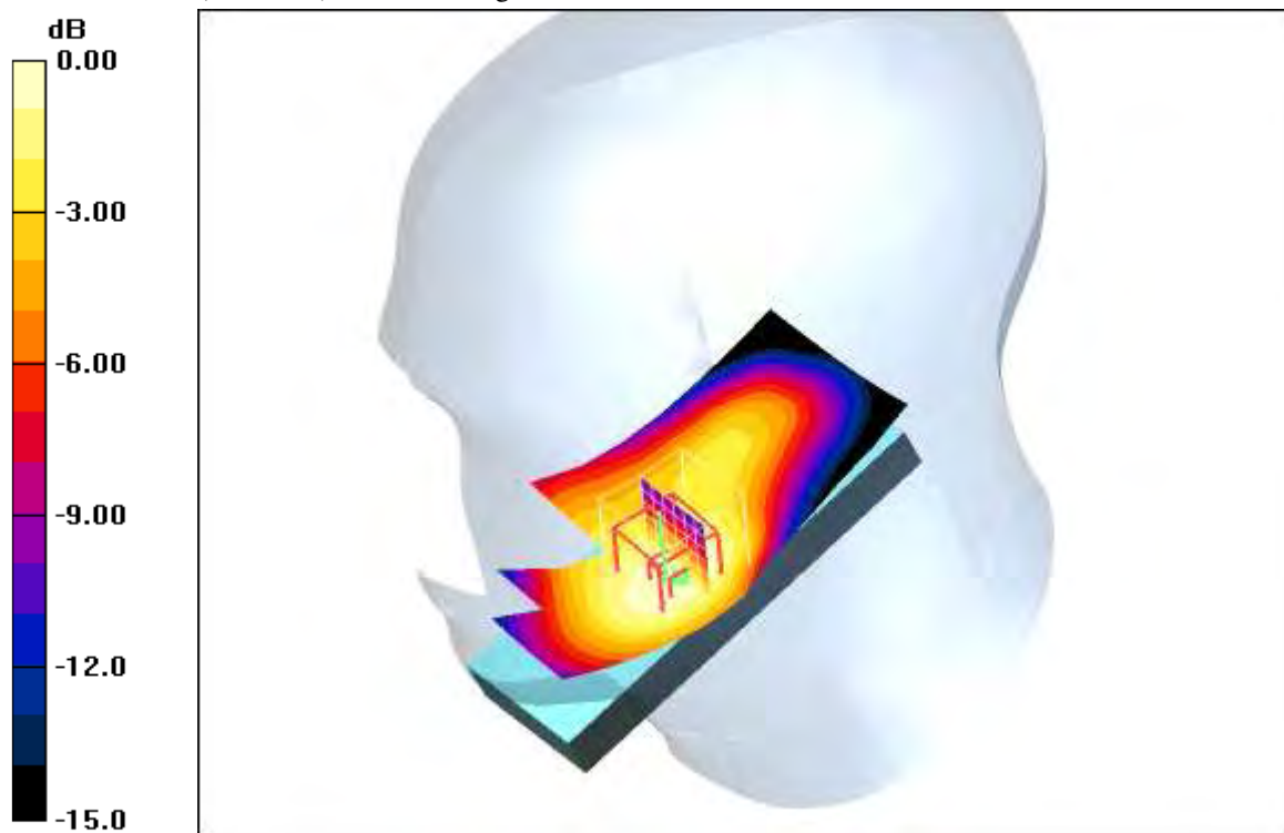
0 dB = 0.381mW/g
