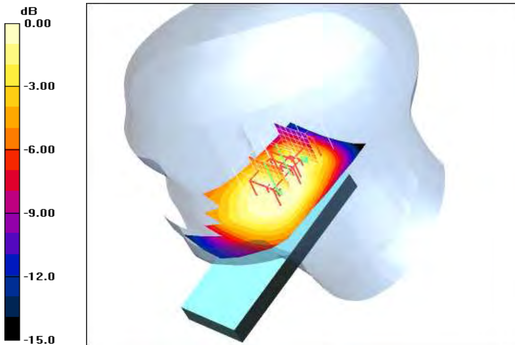
0 dB = 0.228mW/g
