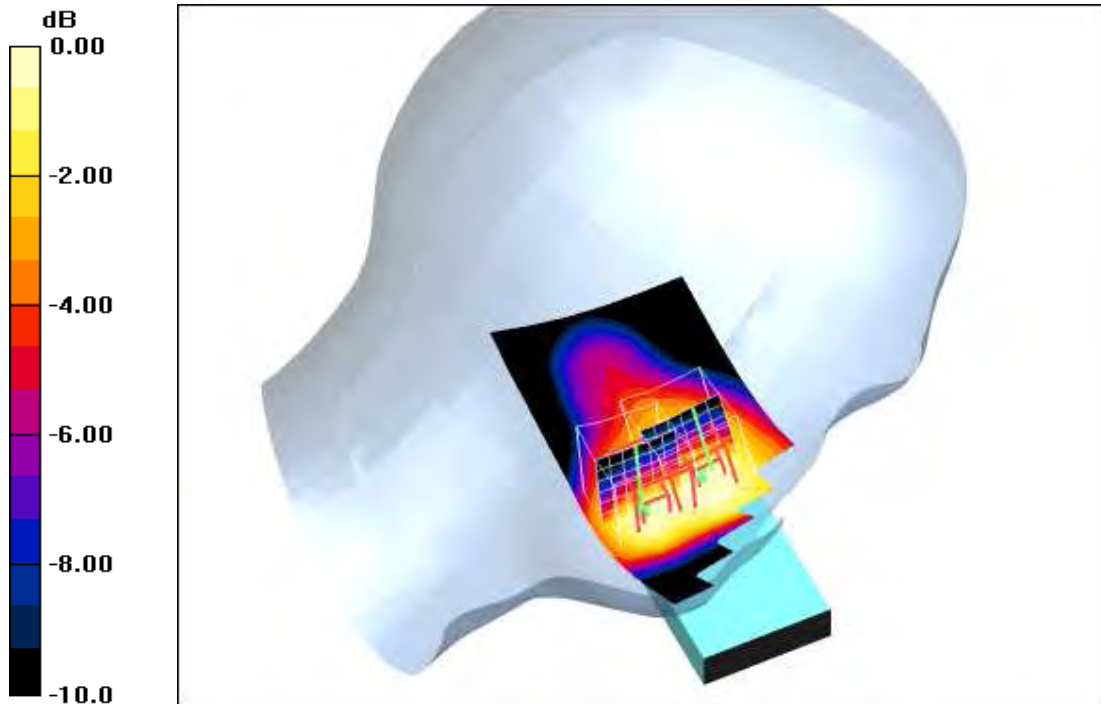
0 dB = 0.239mW/g
