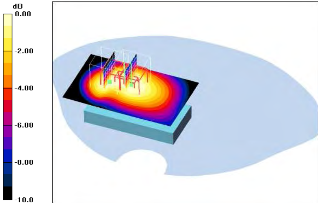
0 dB = 0.332mW/g
