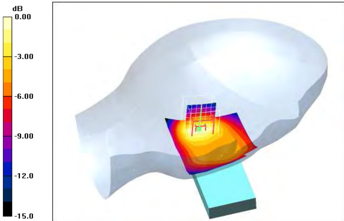
0 dB = 0.183mW/g
