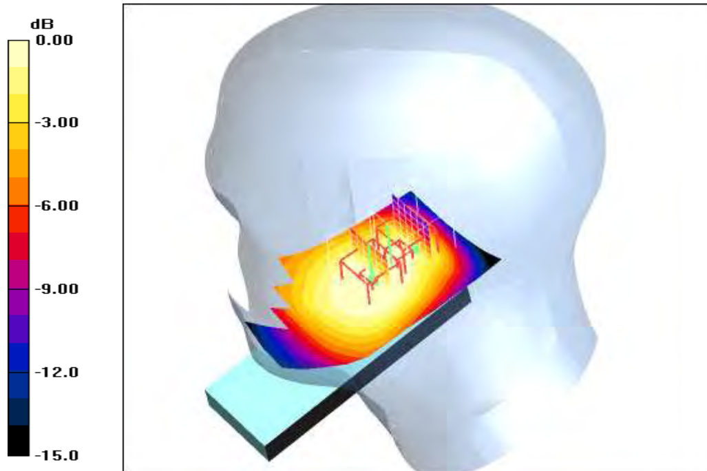
0 dB = 0.265mW/g
