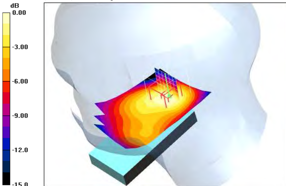
0 dB = 0.114mW/g
