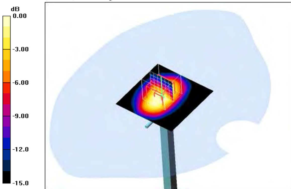
0 dB = 42.1 mW/g
