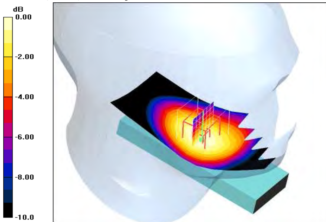
0 dB = 0.653mW/g
