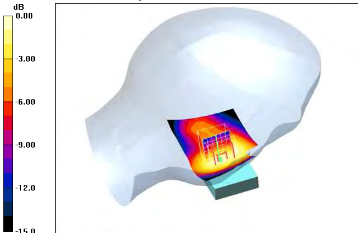
0 dB = 0.447mW/g
