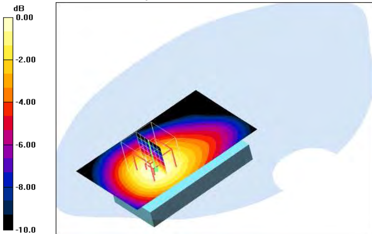
0 dB = 0.217mW/g
