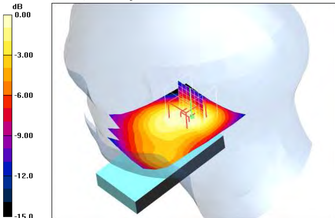
0 dB = 0.198mW/g
