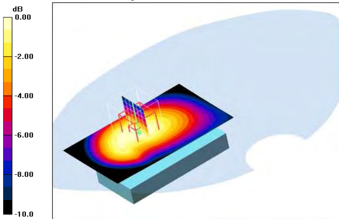
0 dB = 0.273mW/g
