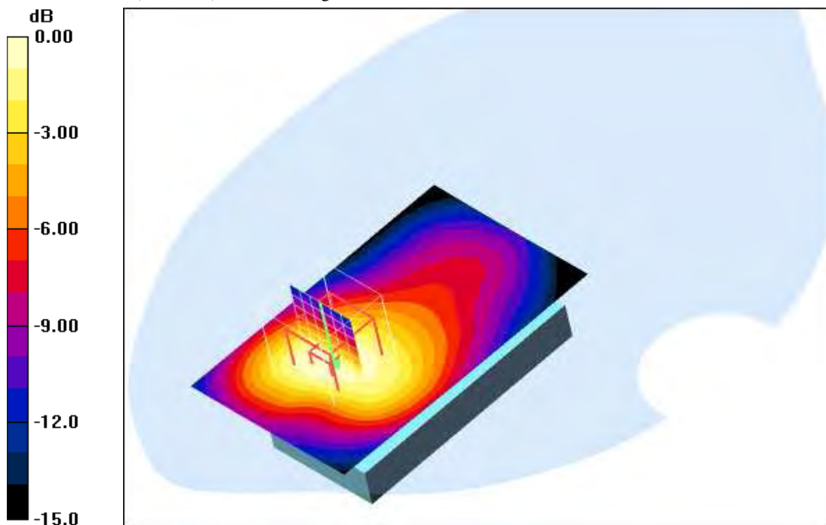
0 dB = 0.282mW/g
