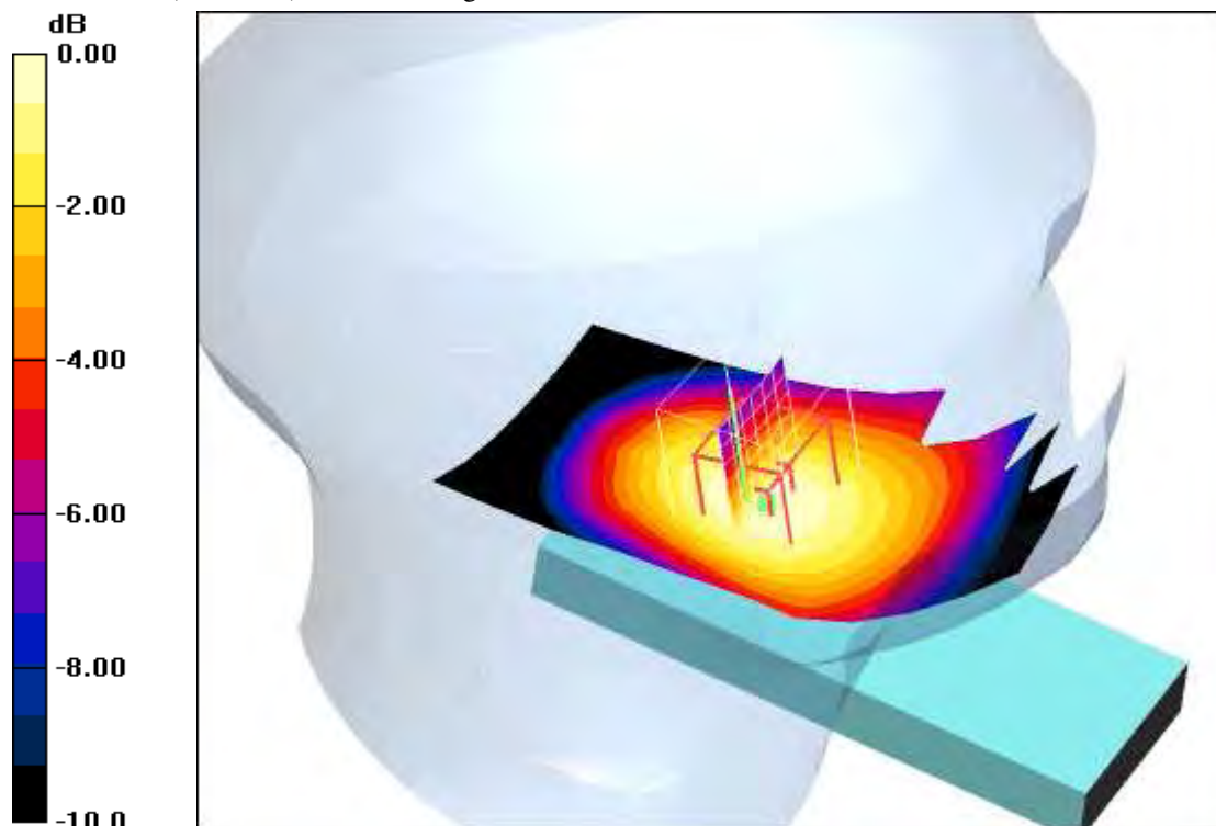
0 dB = 0.253mW/g
