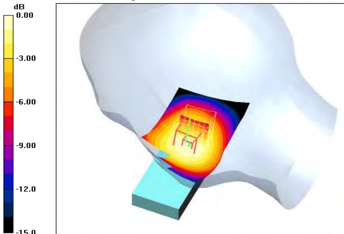
0 dB = 0.465mW/g
