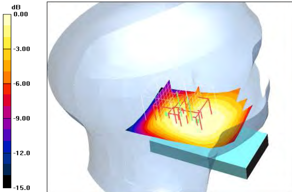
0 dB = 0.125mW/g
