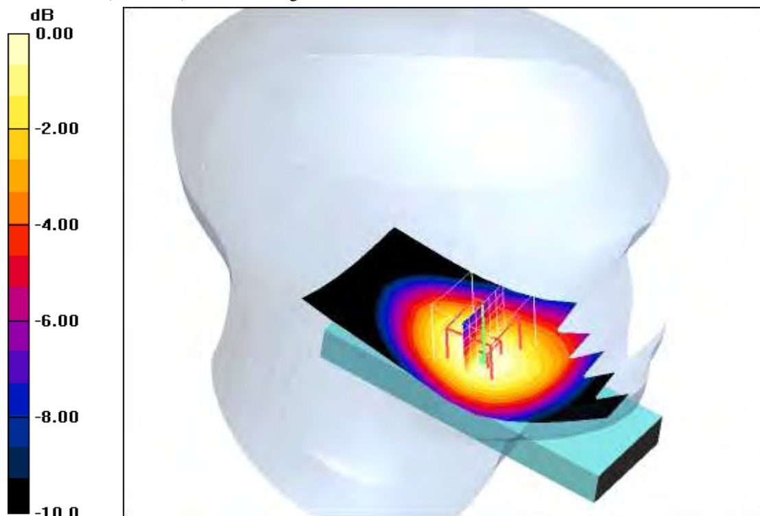
0 dB = 0.732mW/g
