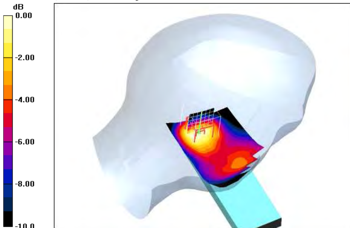
0 dB = 0.252mW/g
