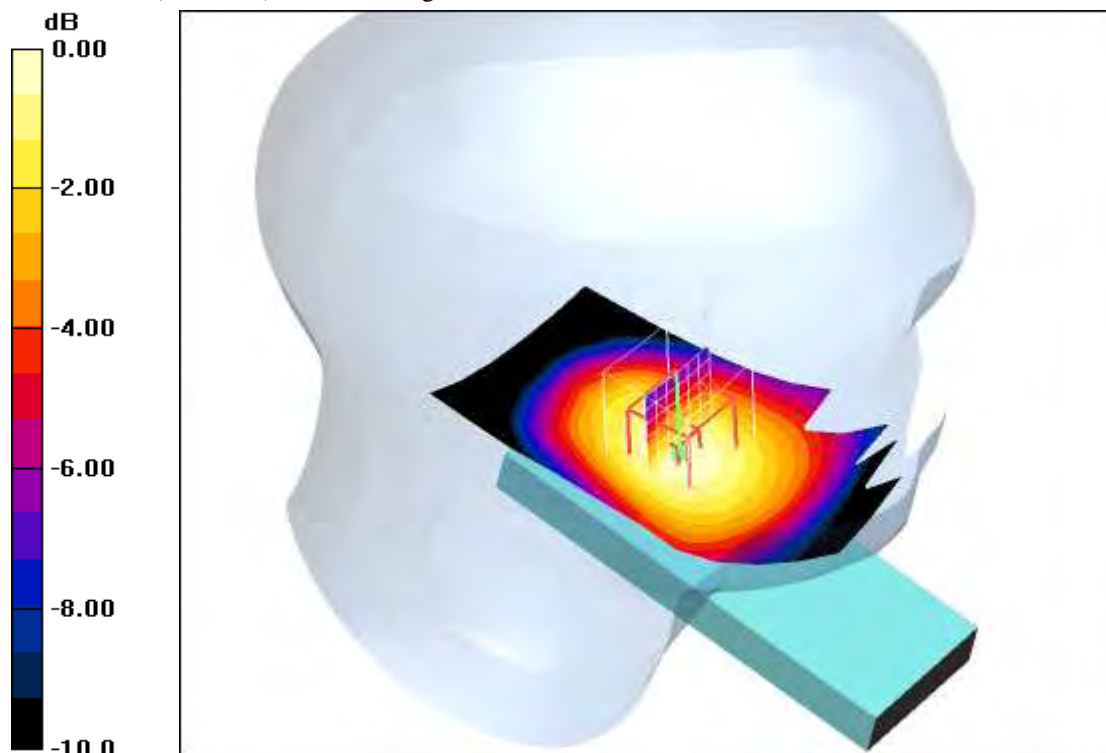
0 dB = 0.307mW/g
