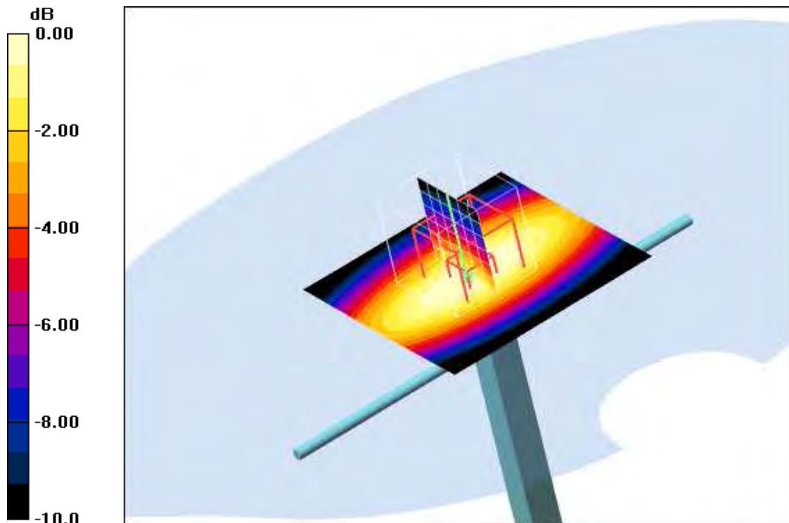
0 dB = 11.5mW/g
