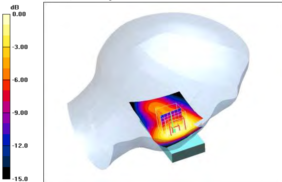
0 dB = 0.602mW/g
