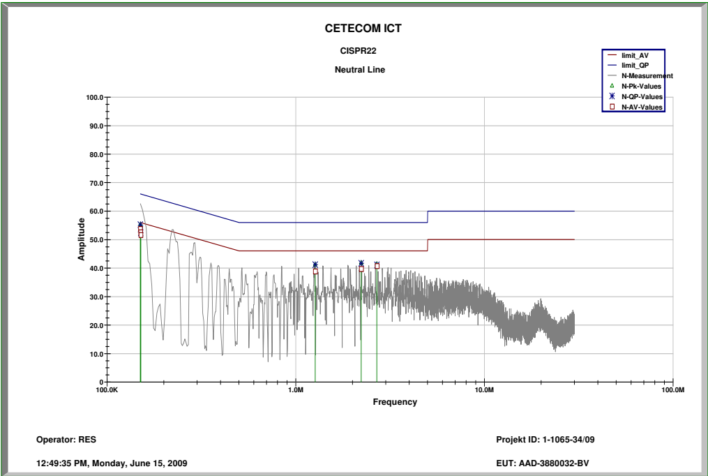
Plot 2: Neutral Line Idle Mode: 150 kHz – 30 MHz
