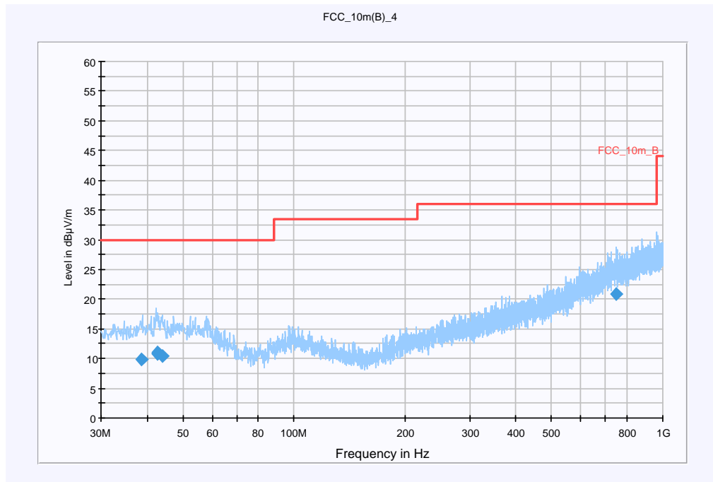
Plot 1: (30 MHz to 1 GHz)
