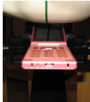
DUT position towards the head: Tilt (touch + 15°) position
