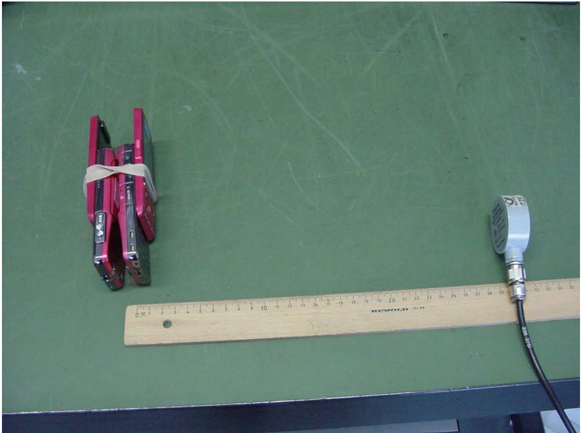
Photo 2 (Radiated Emissions):
