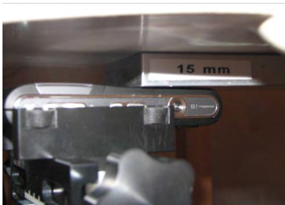
DUT position towards the body with a maximum distance of 15 mm
