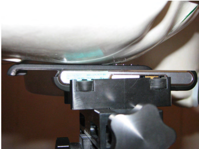
DUT position towards the head with camera cover extracted: Cheek
