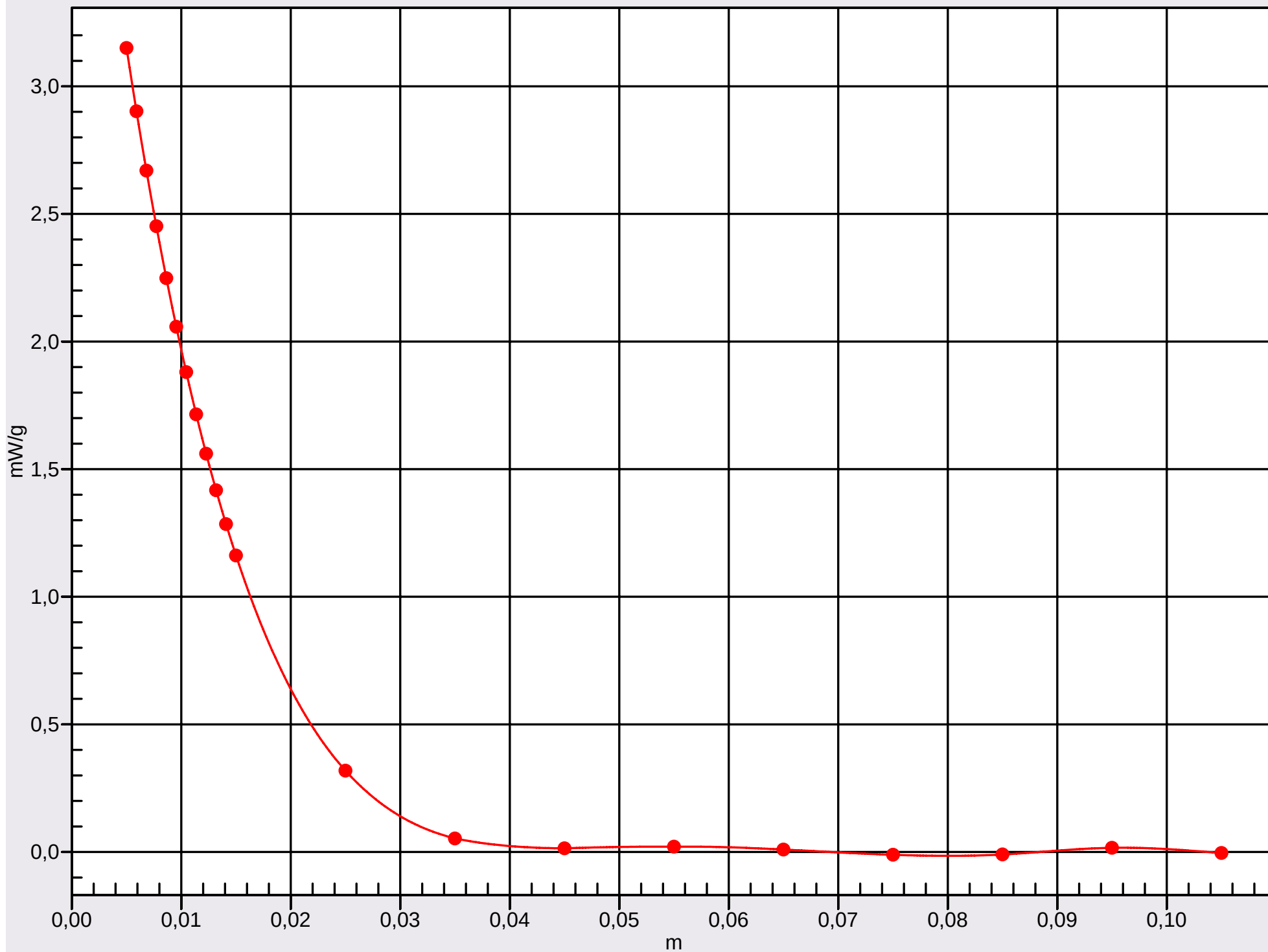
Interpolated SAR(x,y,z,f0) HSL2450; Z Scan: Value Along Z, X=0, Y=0
