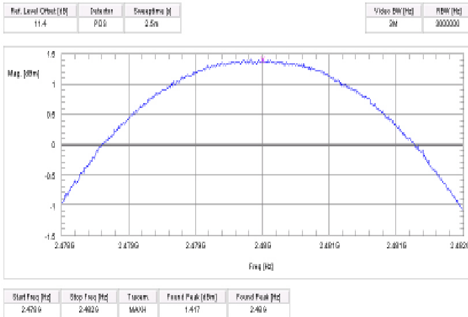
Plot 3 GFSK (conducted)
