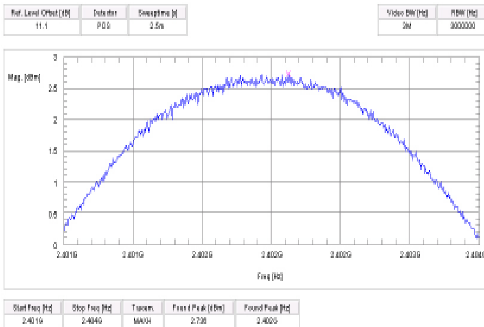
Plot 4 Pi/4 DQPSK (conducted)
