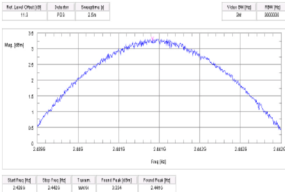
Plot 8 8DPSK (conducted)
