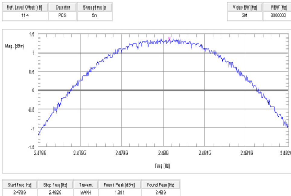
Plot 6 Pi/4 DQPSK (conducted)
