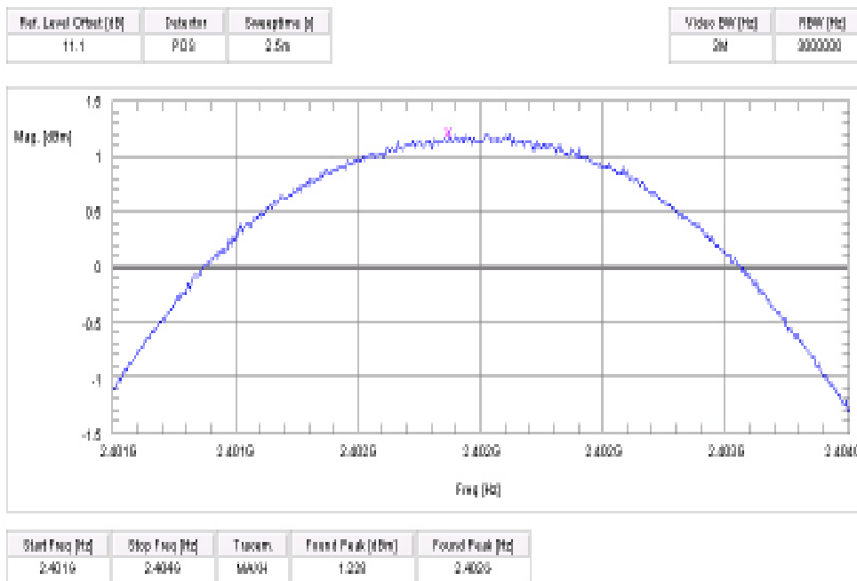
Plot 2 GFSK (conducted)
