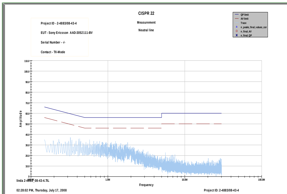
Plot 2: TX mode neutral line
