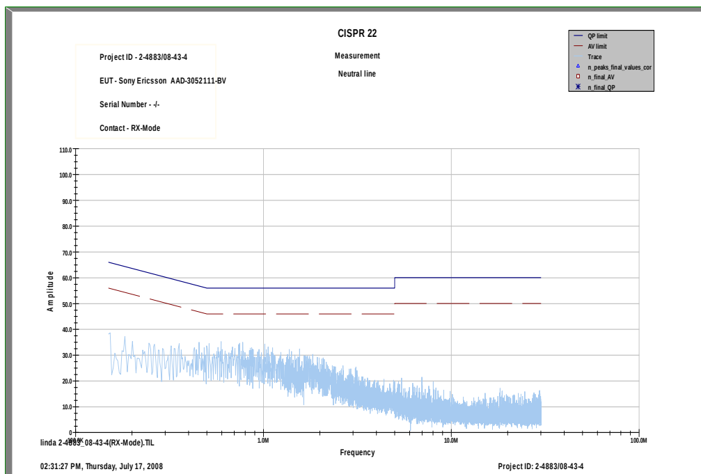
Plot 4: RX mode neutral line
