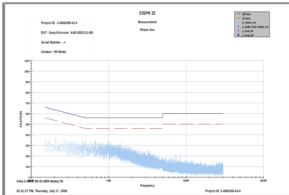
Plot 3: RX mode phase line
