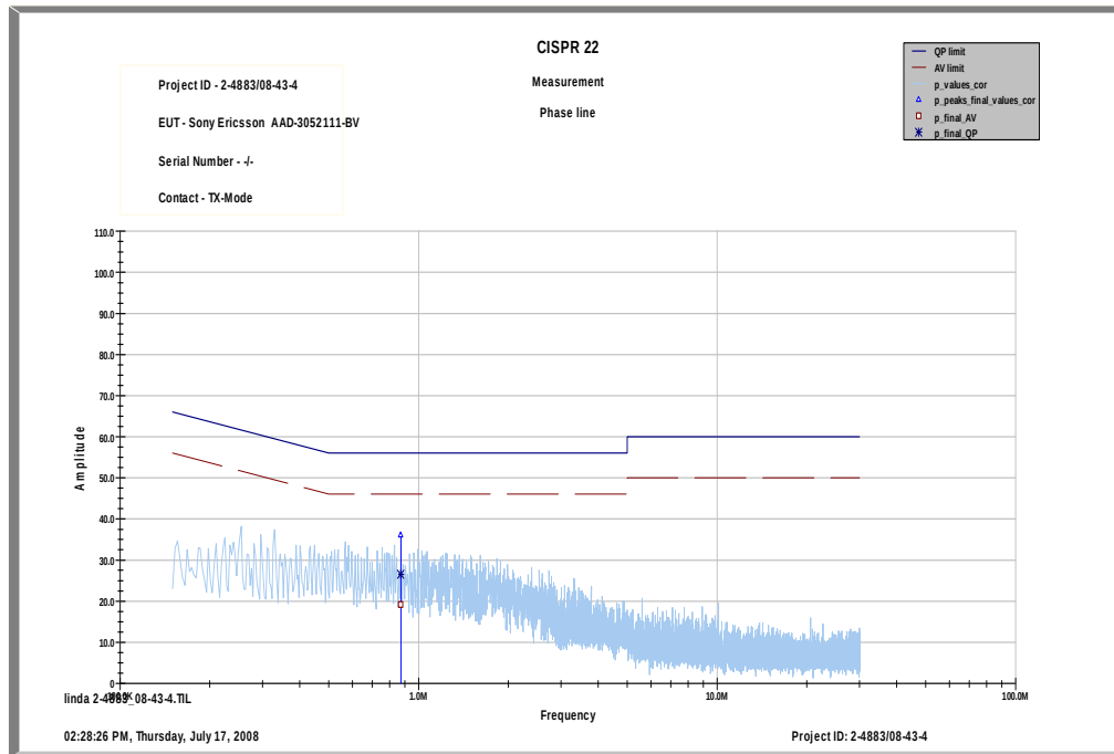
Plot 1: TX mode phase line
