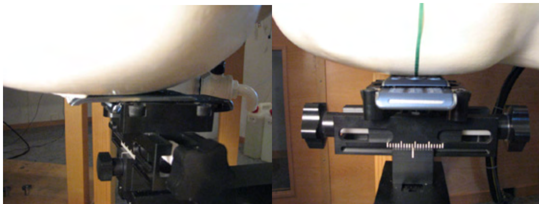
DUT position towards the head: Cheek (touch) position open
