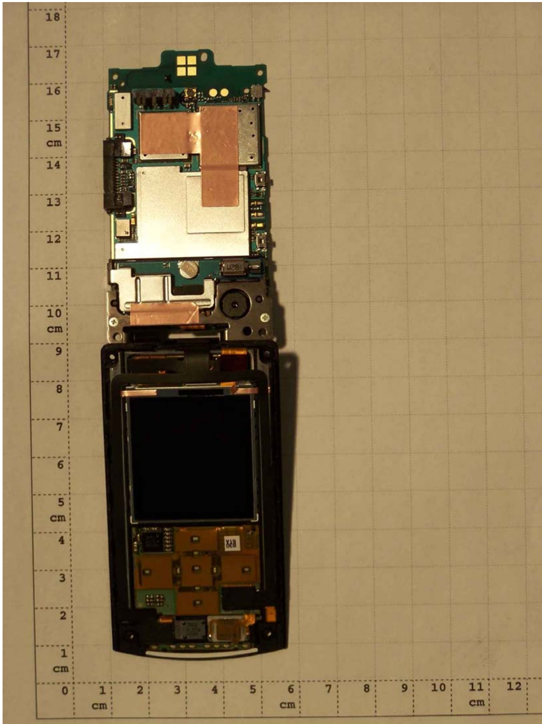
Photograph 13: Inside view of EUT A
