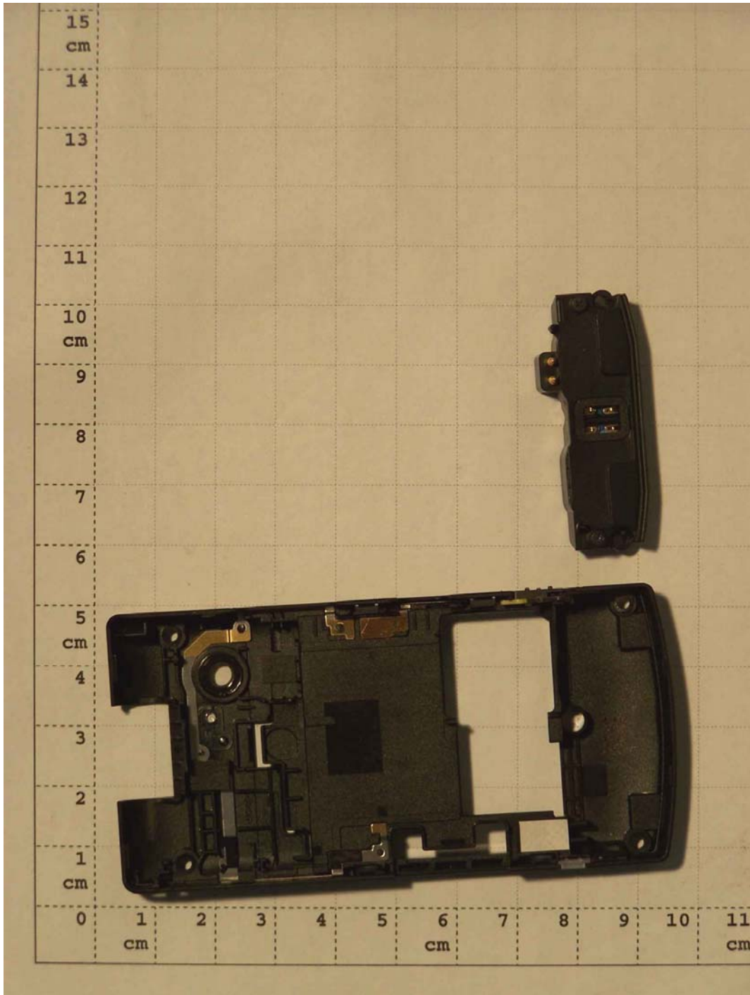
Photograph 14: Inside view EUT A: Antenna + cover
