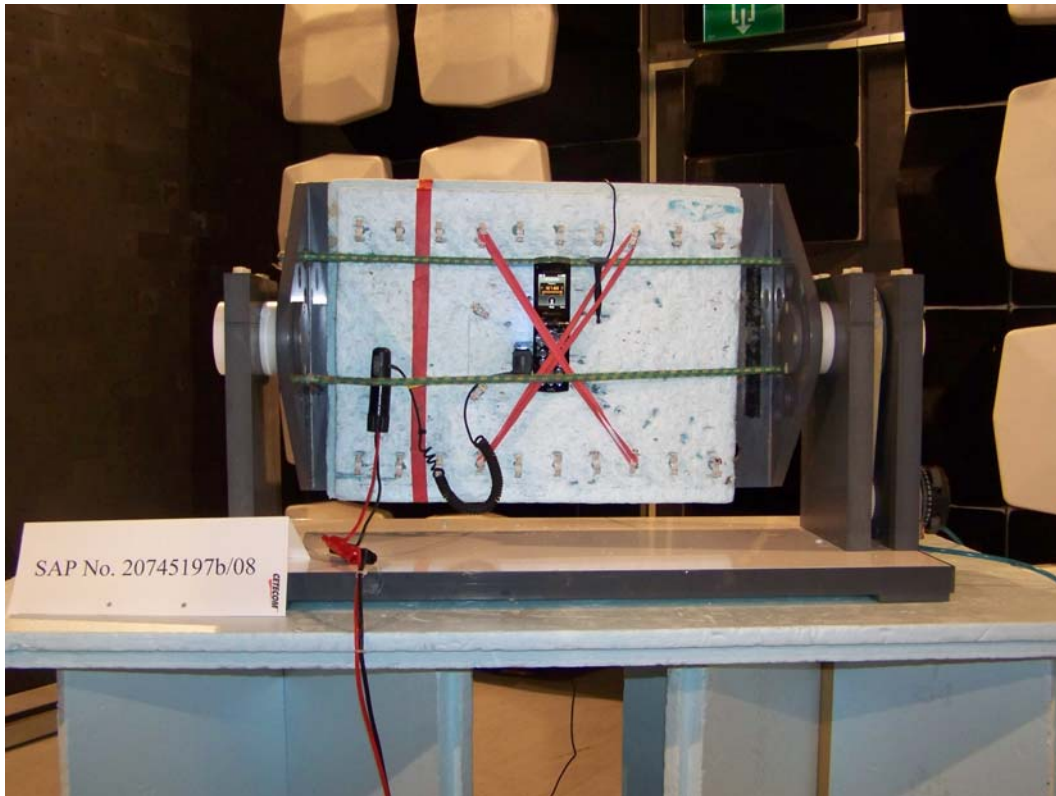
Photograph 3: Measurement set-up: Radiated field strength
