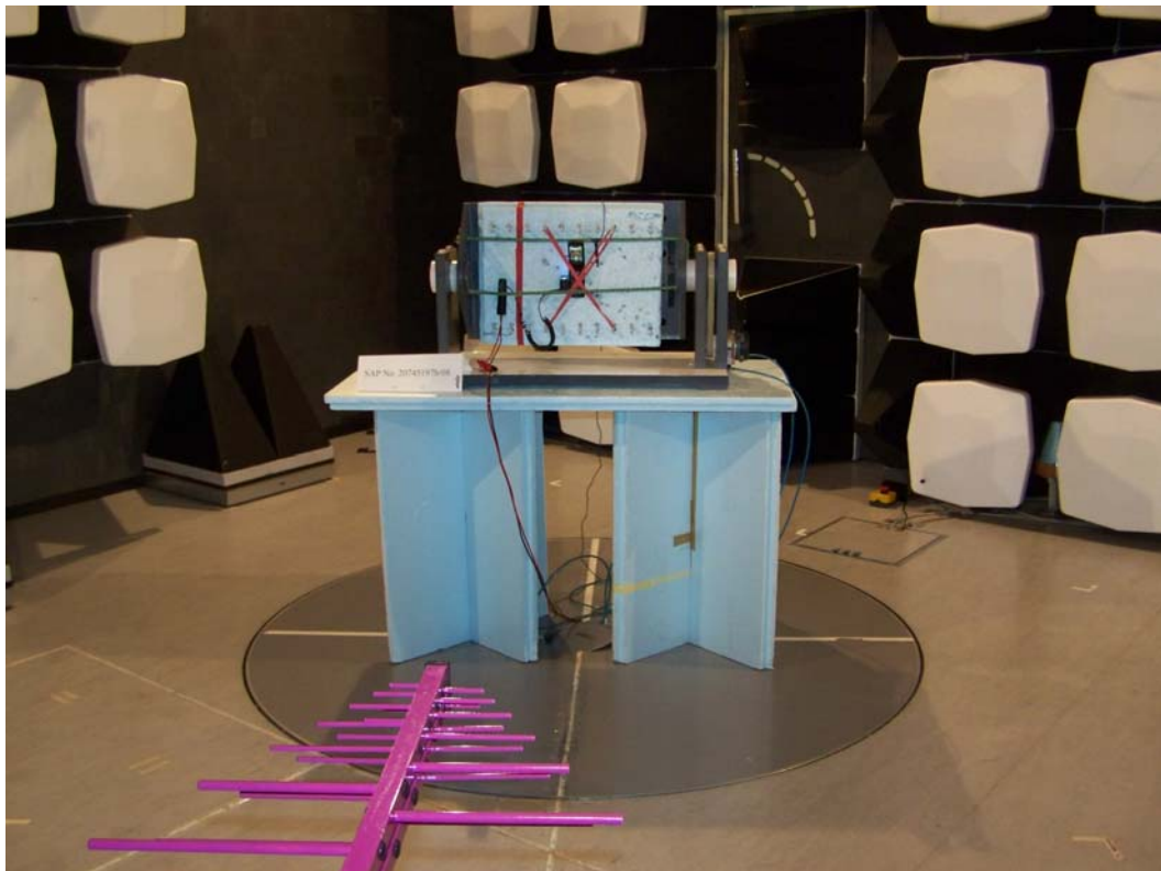
Photograph 4: Measurement set-up: Radiated field strength
