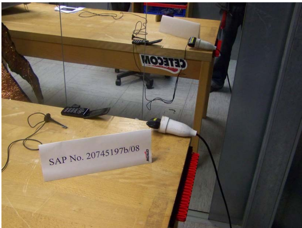
Photograph 2: Measurement set-up: conducted emissions on AC-Power lines
