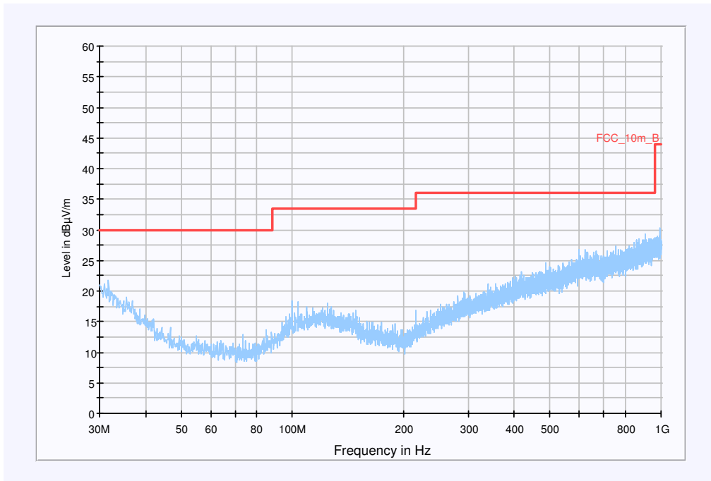
Plot 5: 0.03 - 1 GHz vertical/horizontal (middle channel)
