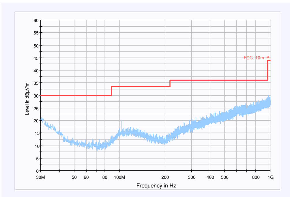
Plot 8: 0.03 - 1 GHz vertical/horizontal (highest channel)
