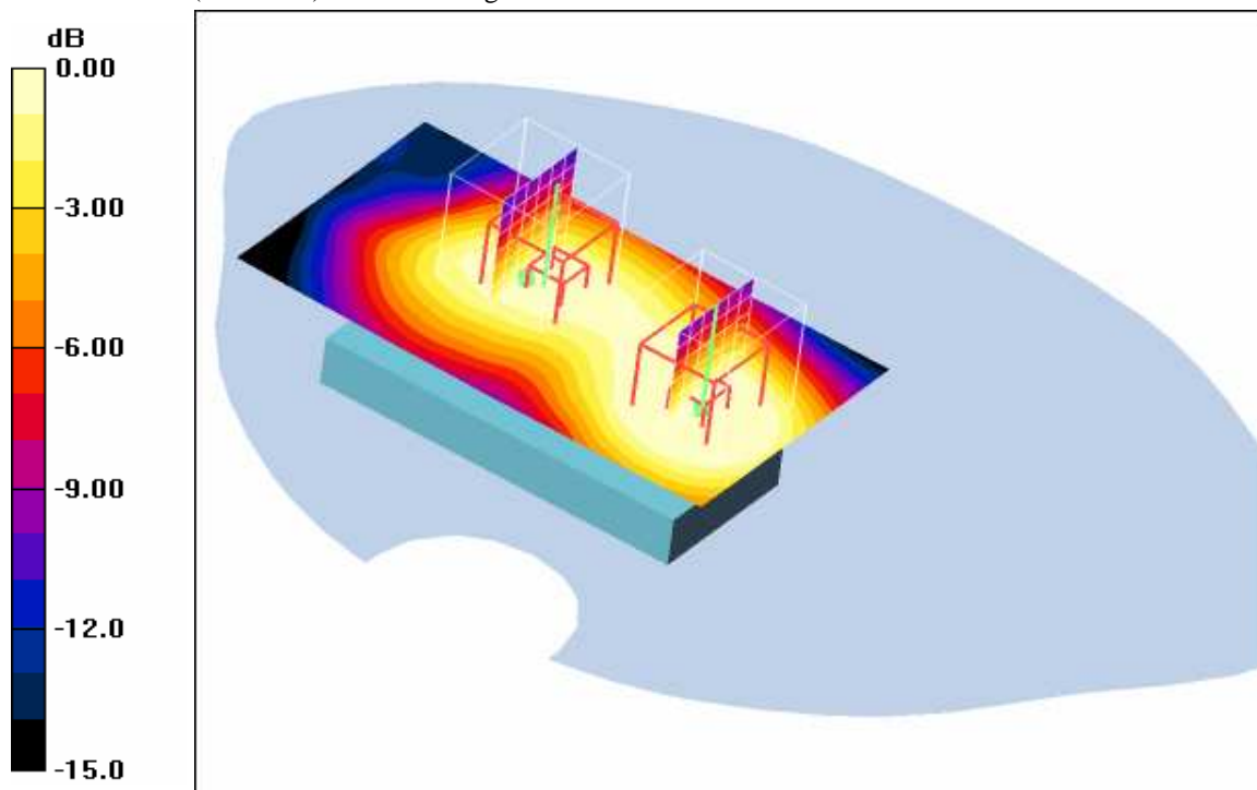
0 dB = 0.164mW/g
