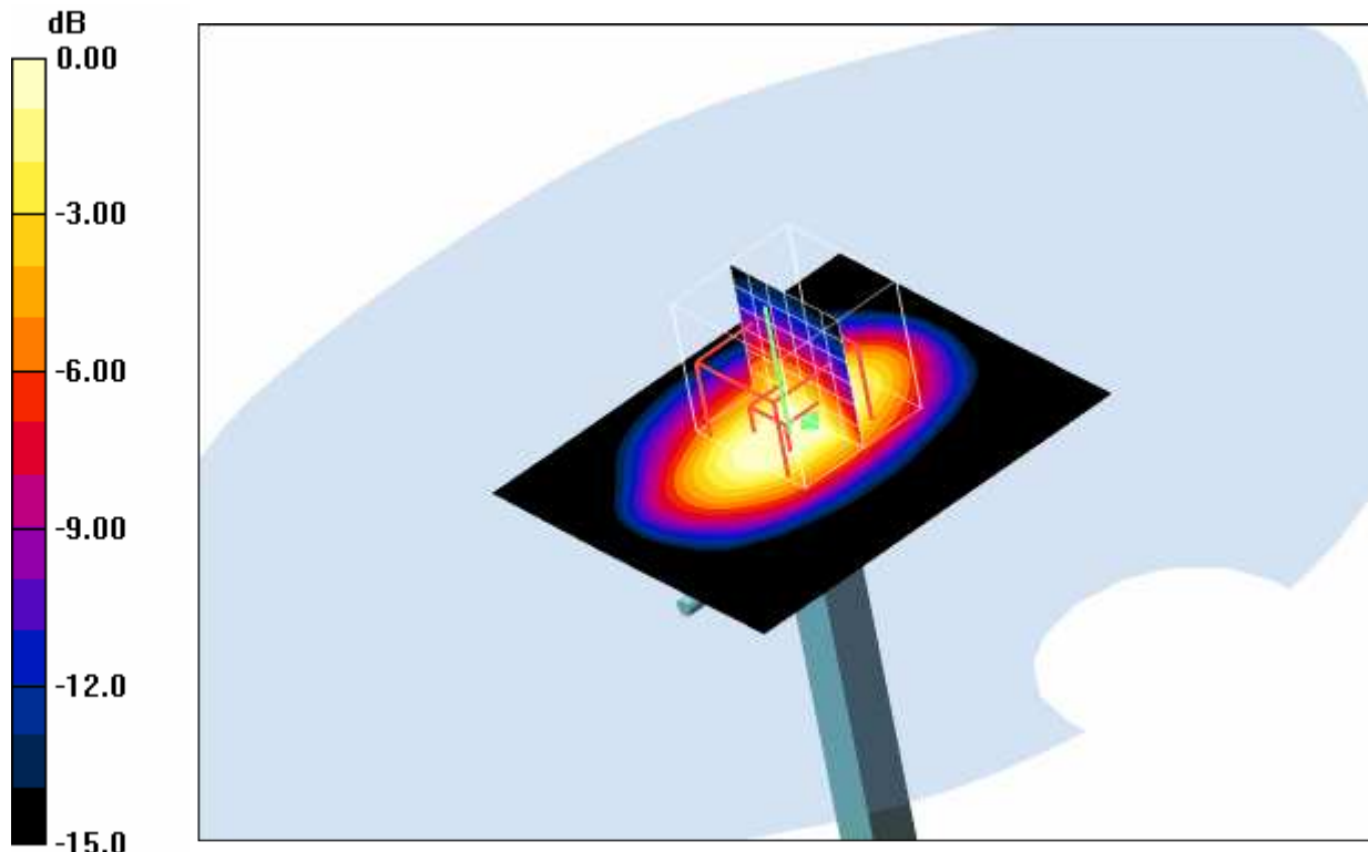
0 dB = 42.3mW/g
