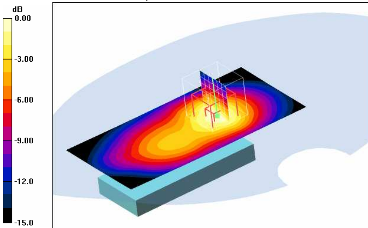
0 dB = 0.691mW/g
