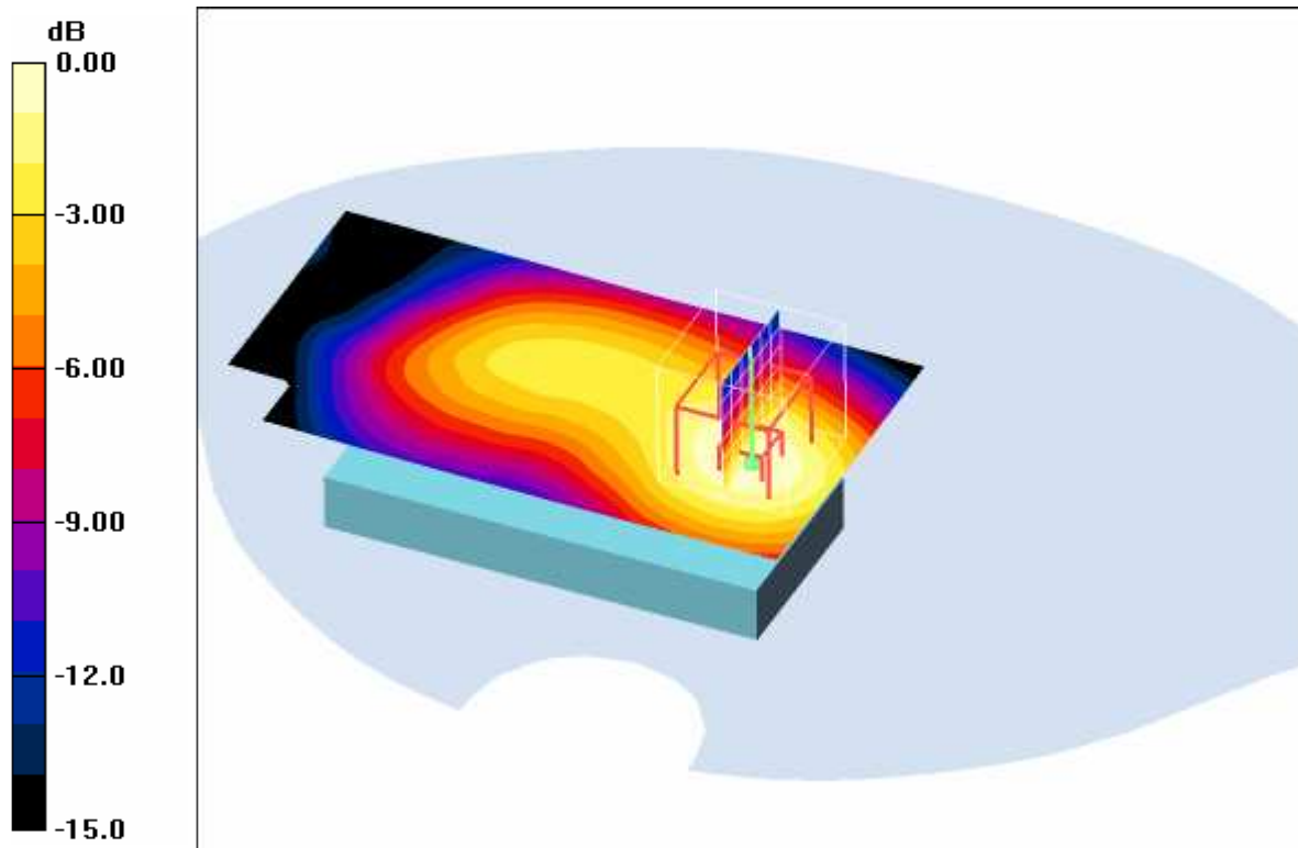
0 dB = 0.320mW/g
