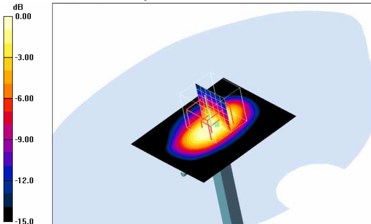
0 dB = 43.6mW/g
