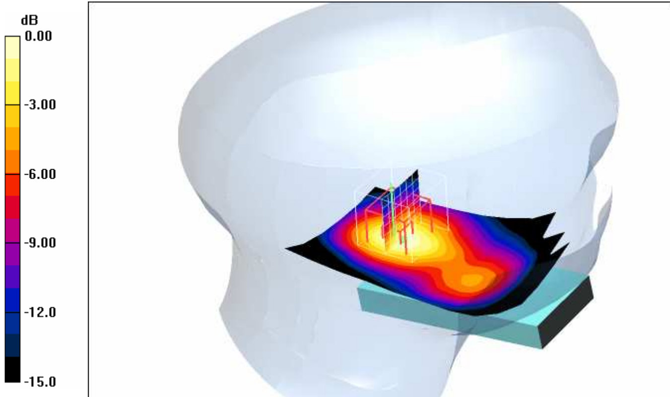
0 dB = 1.11mW/g
