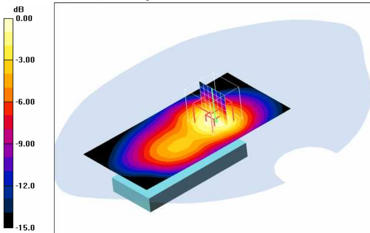
0 dB = 0.888mW/g
