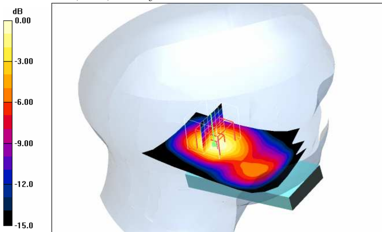
0 dB = 1.52mW/g
