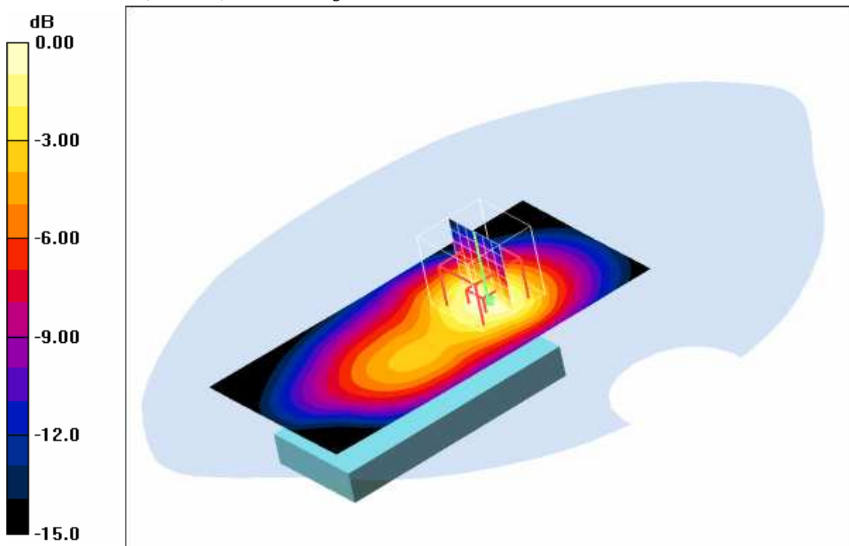
0 dB = 0.857mW/g
