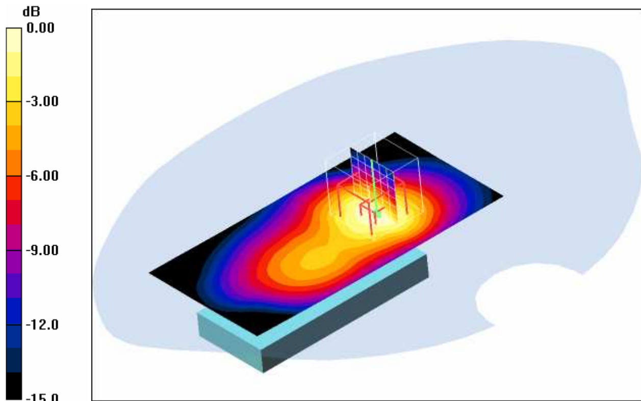
0 dB = 0.632mW/g
