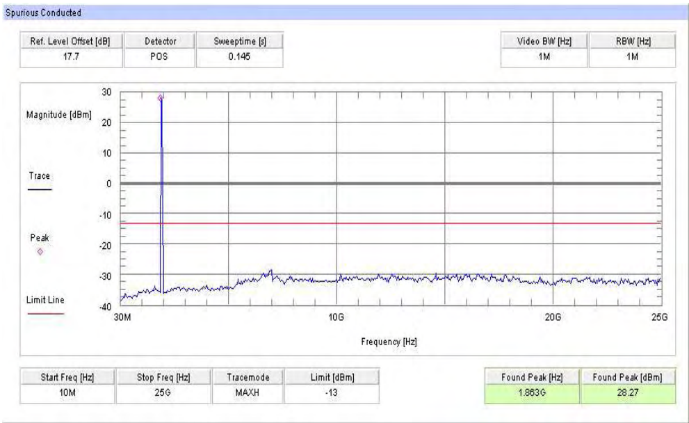
Plot 3: Channel 810 (10 MHz - 25 GHz)
