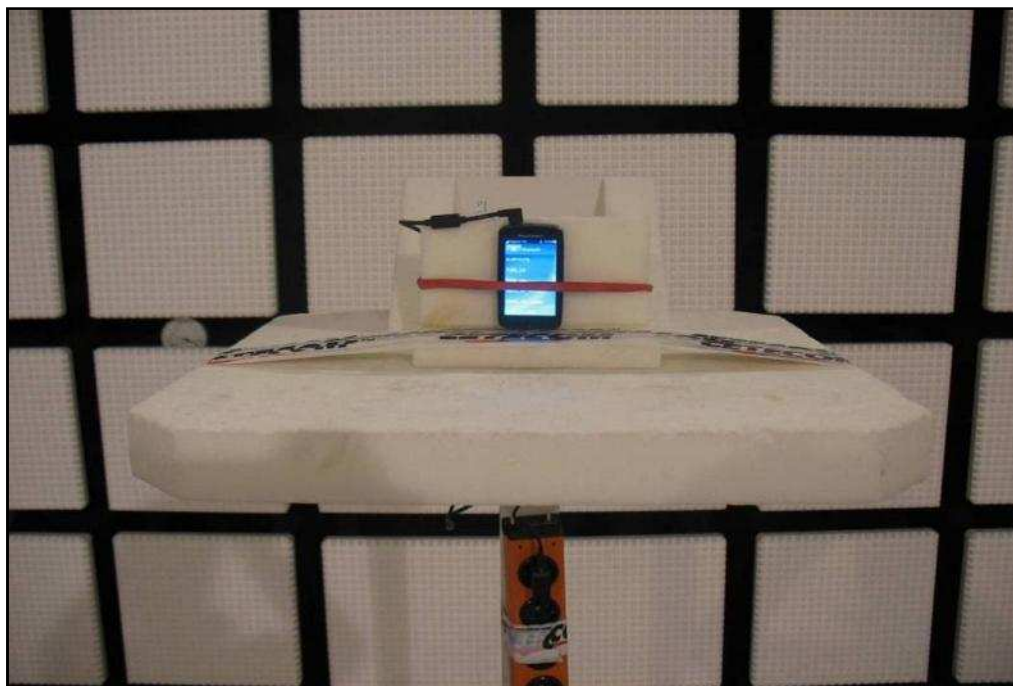
Photo 4: chamber C
