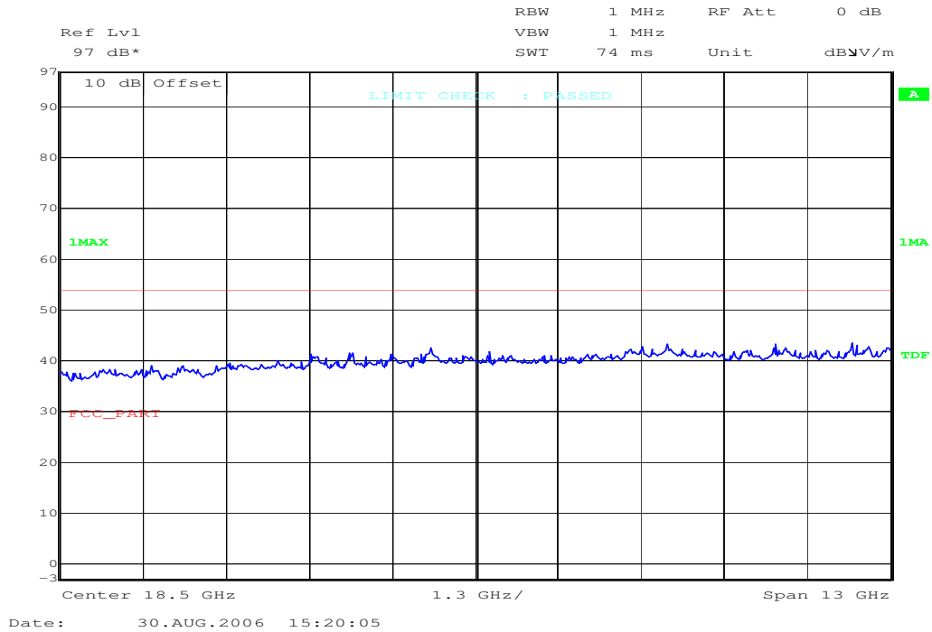
Plot : 12- 25 GHz vertical worst case (valid for all three channels)
