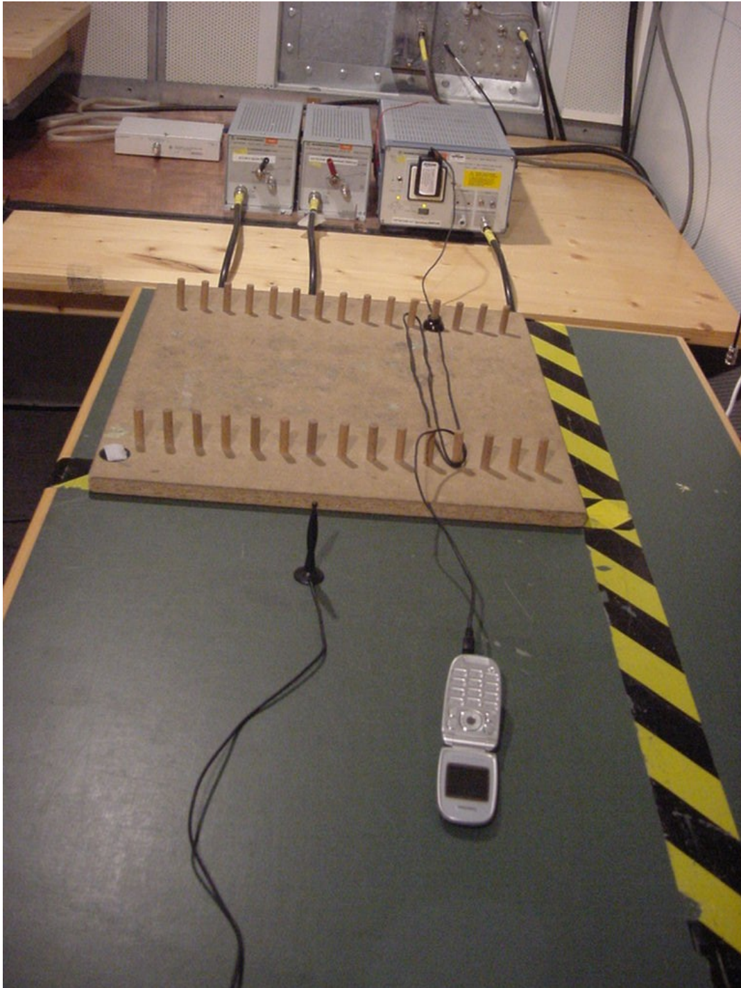
Photo 3 (Conducted Emissions):
