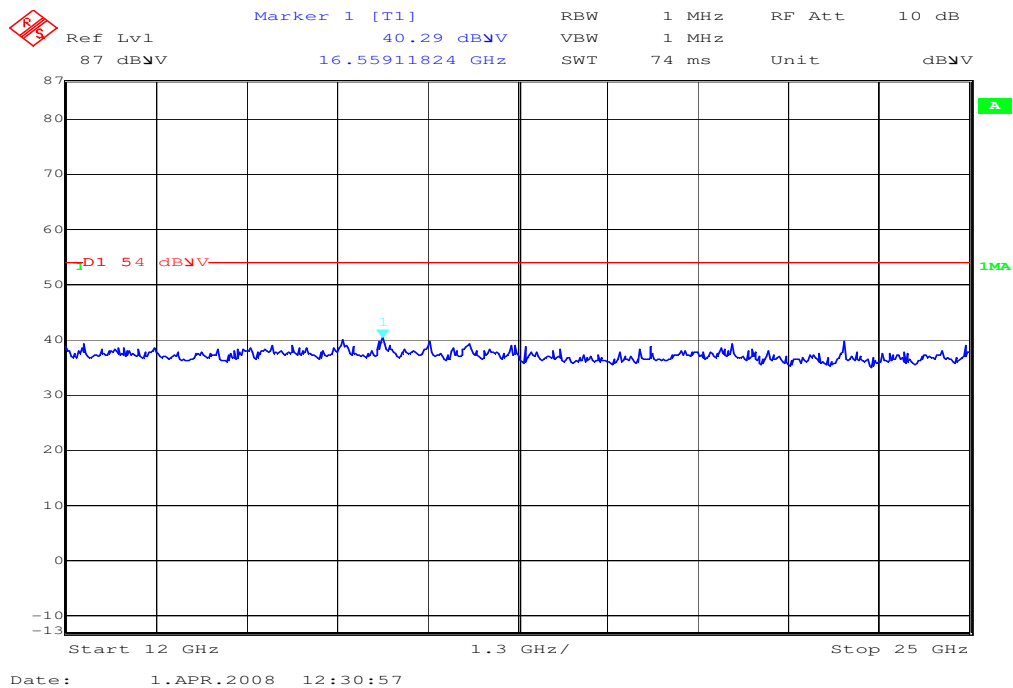
Plot: 12 - 25 GHz vertical/horizontal (valid for all channels)
