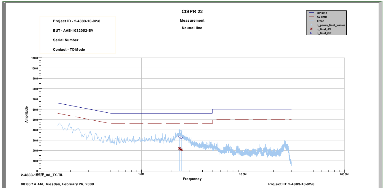
Plot 2: Traffic Mode - 1900 MHz: 150 kHz – 30 MHz
