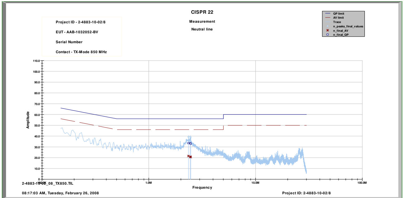
Plot 2: Traffic Mode - 850 MHz: 150 kHz – 30 MHz
