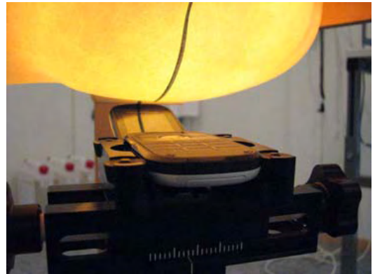
Device position towards the head: Tilt (cheek+15deg) phone position
