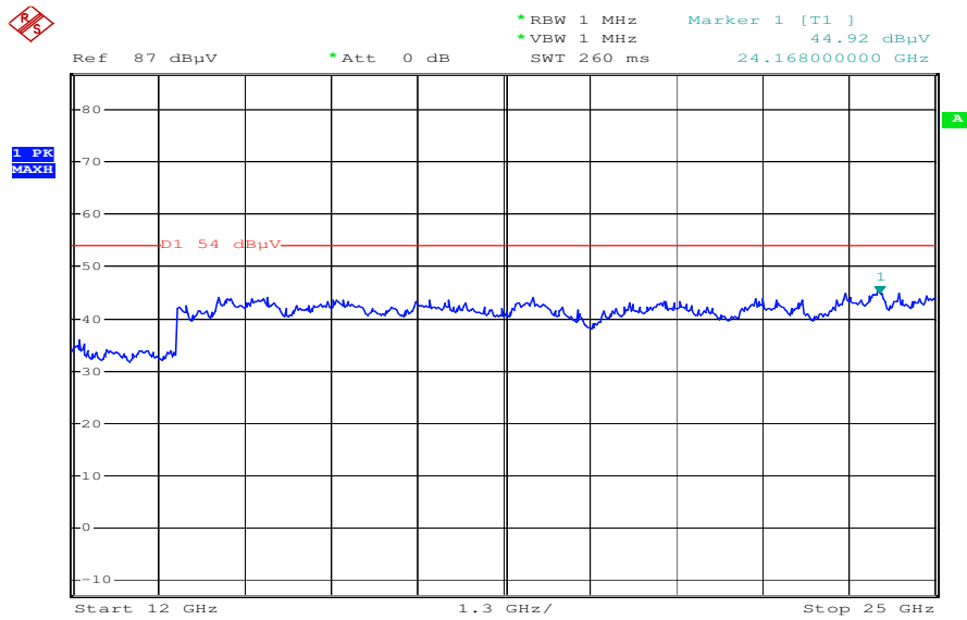
Plot 3: GSM 850 RX (12 GHz to 25 GHz)
