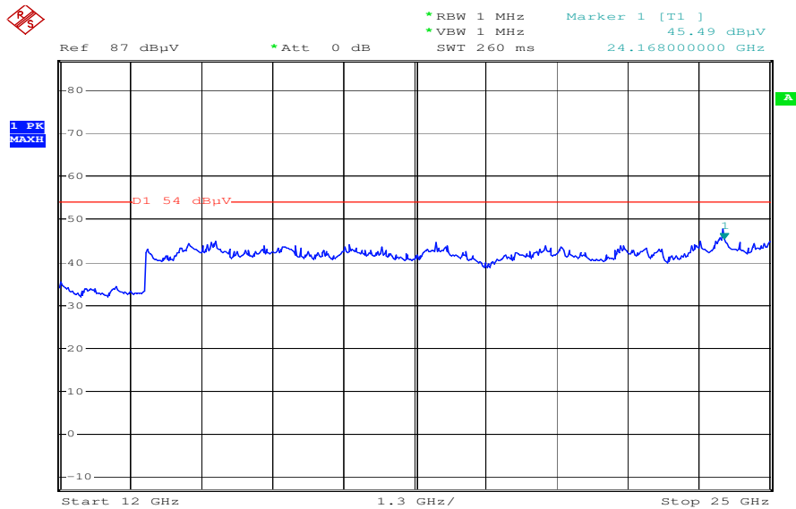
Plot 3: PCS 1900 RX (12 GHz to 25 GHz)
