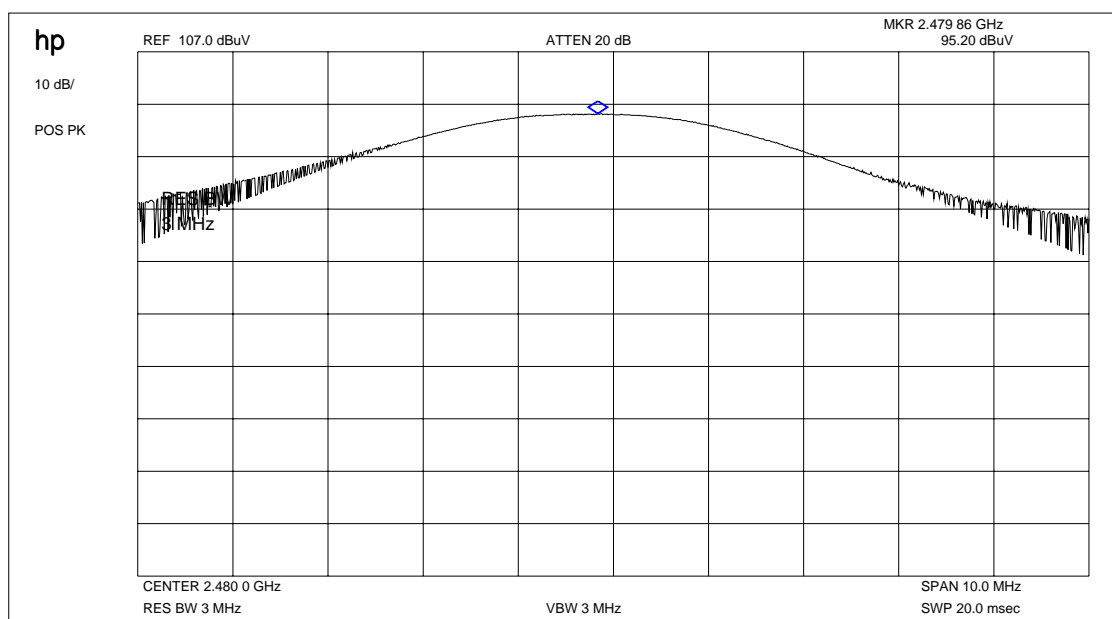
Plot 1 : Max field strength in 3m distance (single frequency)
