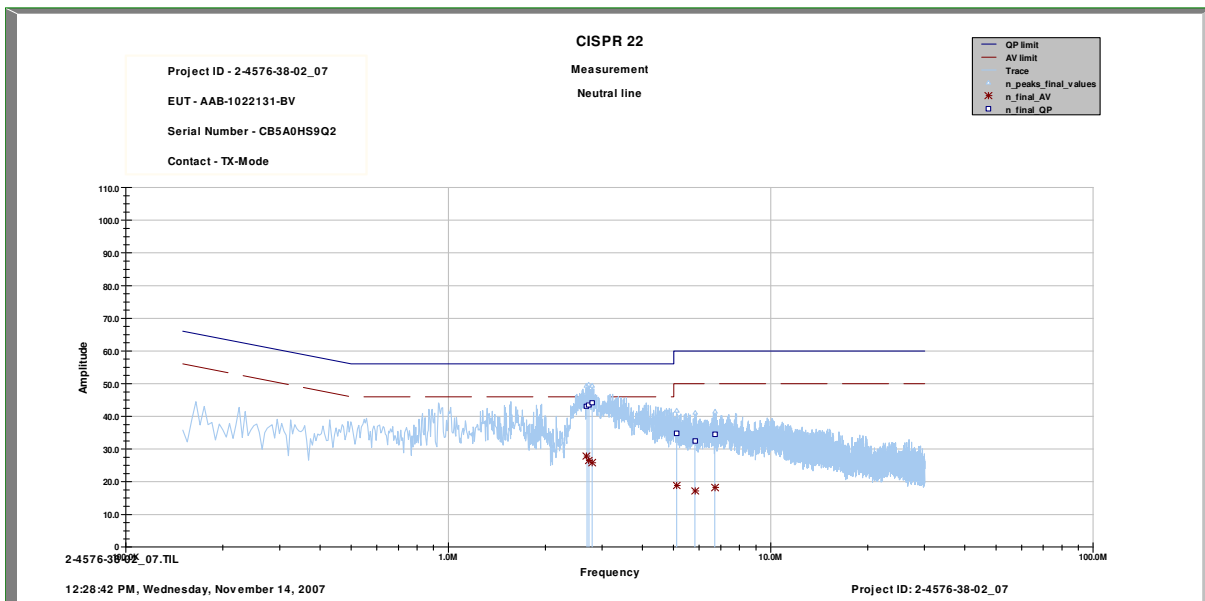
Plot 2: Traffic Mode : 150 kHz – 30 MHz
