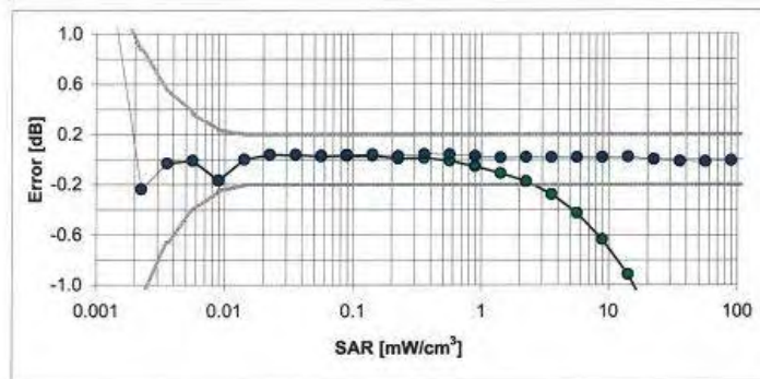
Uncertainty of Linearity Assessment: \pm 0.6\% ( k=2 )
