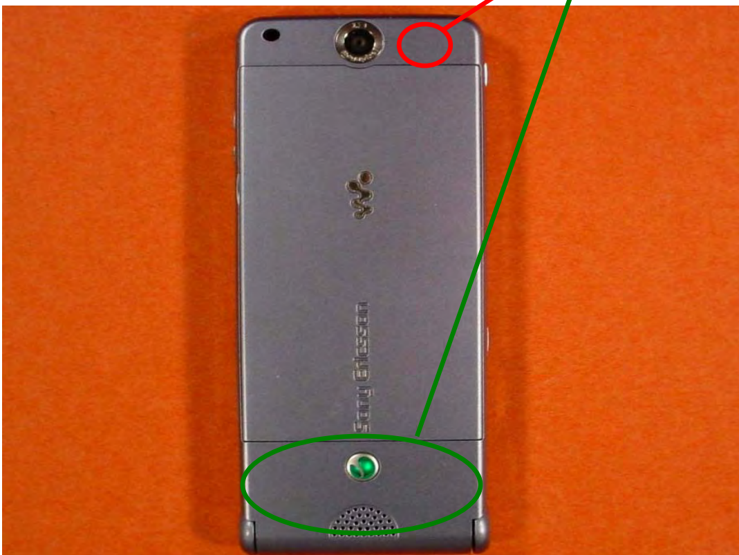
Photo 6: DUT - rear view (with antenna positions BT and GSM)
