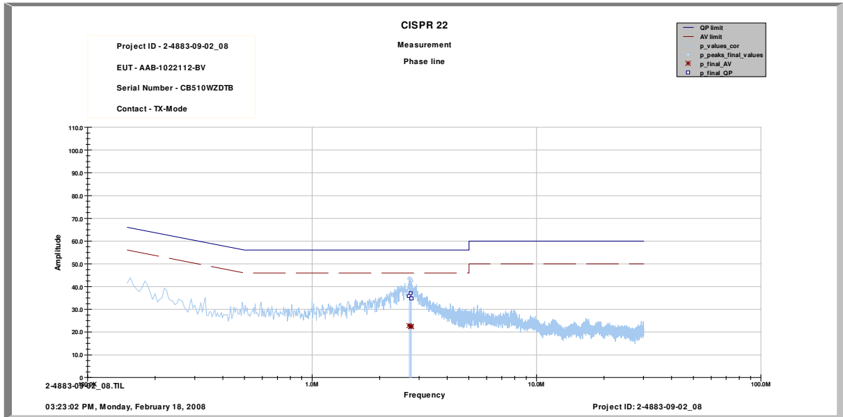
Plot 3: 150 kHz – 30 MHz (Phase Line)
