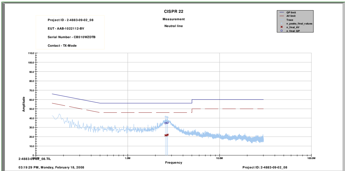
Plot 4: 150 kHz – 30 MHz (Neutral Line)
