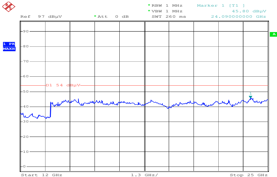
Plot 4: RX (12 GHz to 25 GHz)
