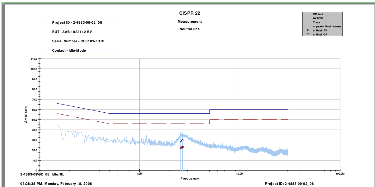
Plot 2: 150 kHz – 30 MHz (Neutral Line)
