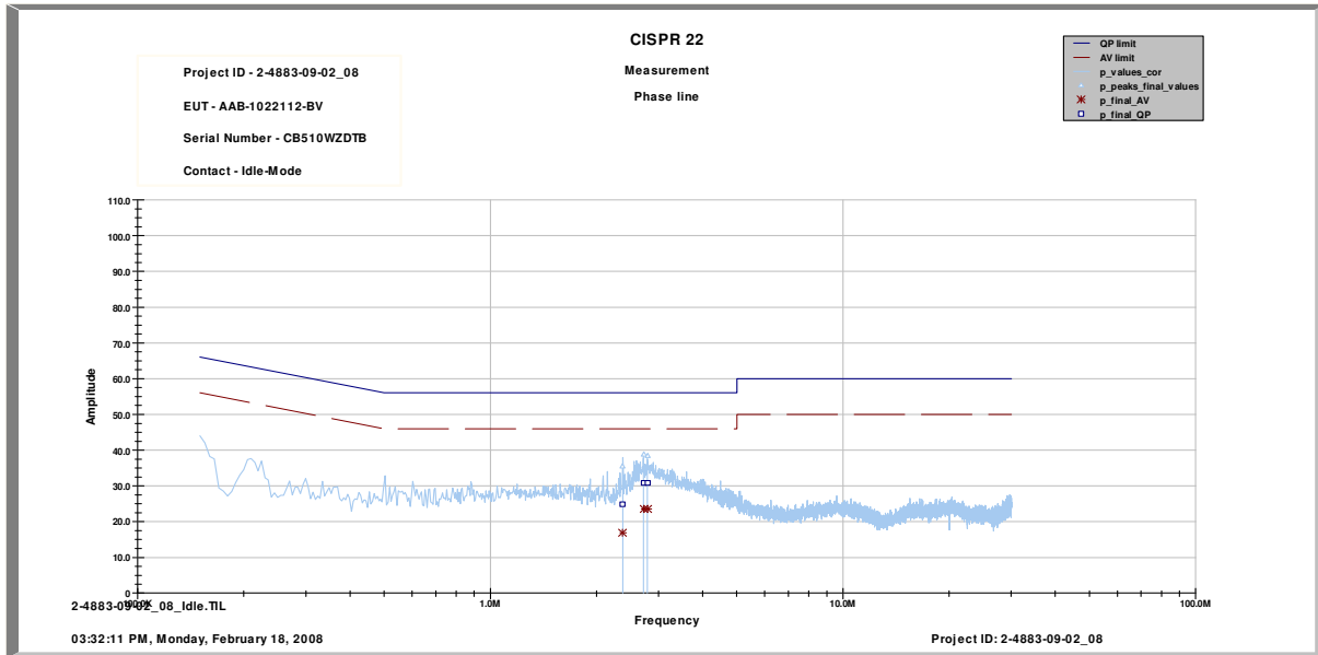
Plot 1: 150 kHz – 30 MHz (Phase Line)
