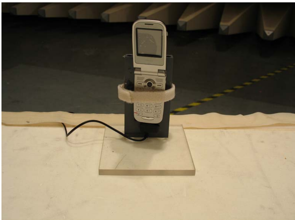
Photo 2: Radiated Emissions
