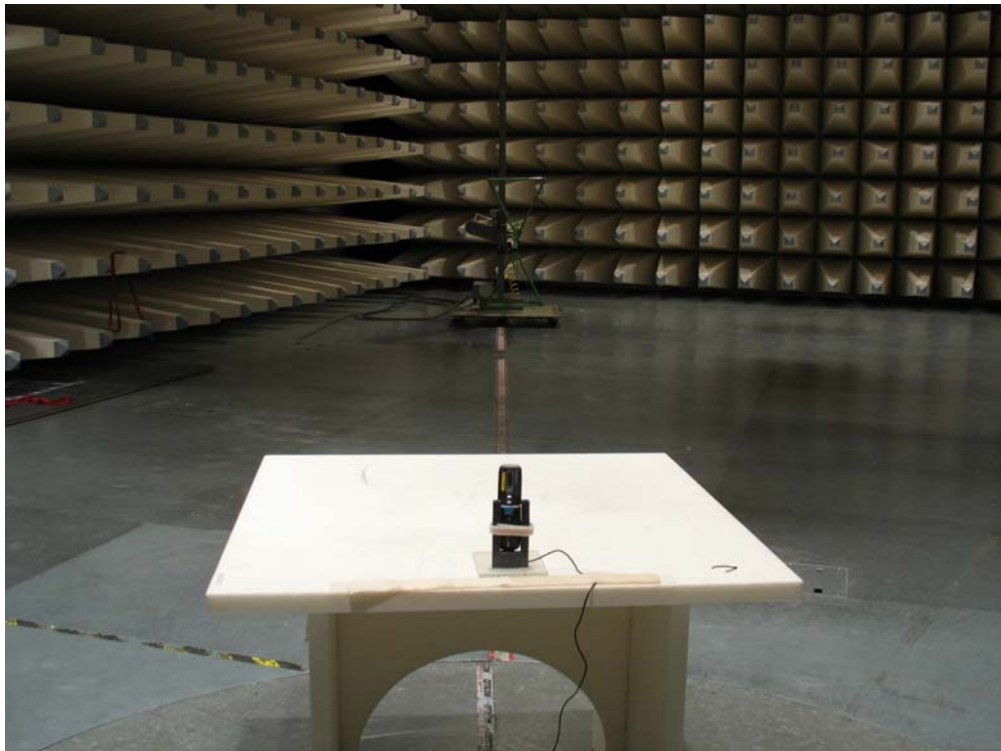
Photo 1: Radiated Emissions
