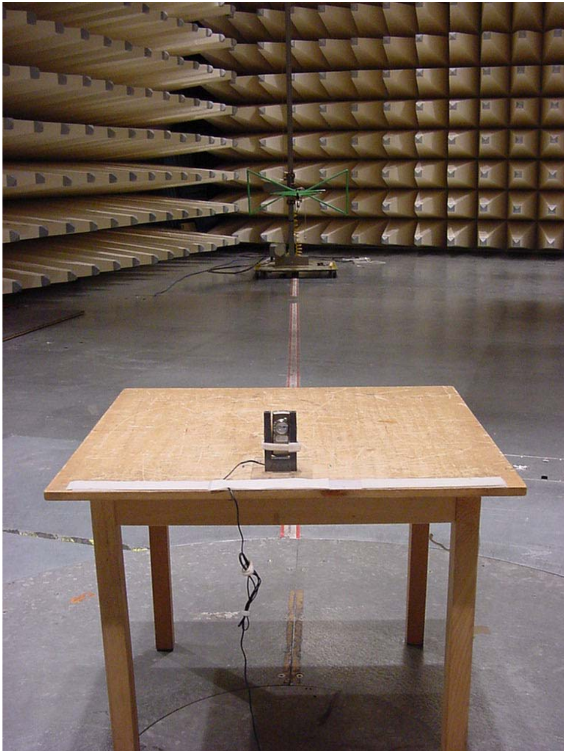
Photo 1: Radiated Emissions
