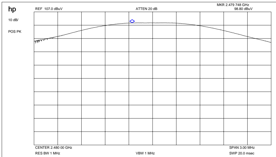
Plot 1 : Max field strength in 3m distance (single frequency)
