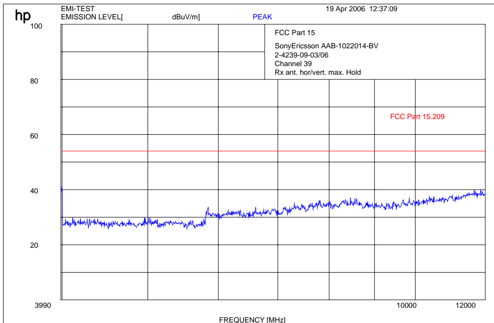
Plot : 4- 12 GHz vertical/horizontal (middle channel)
