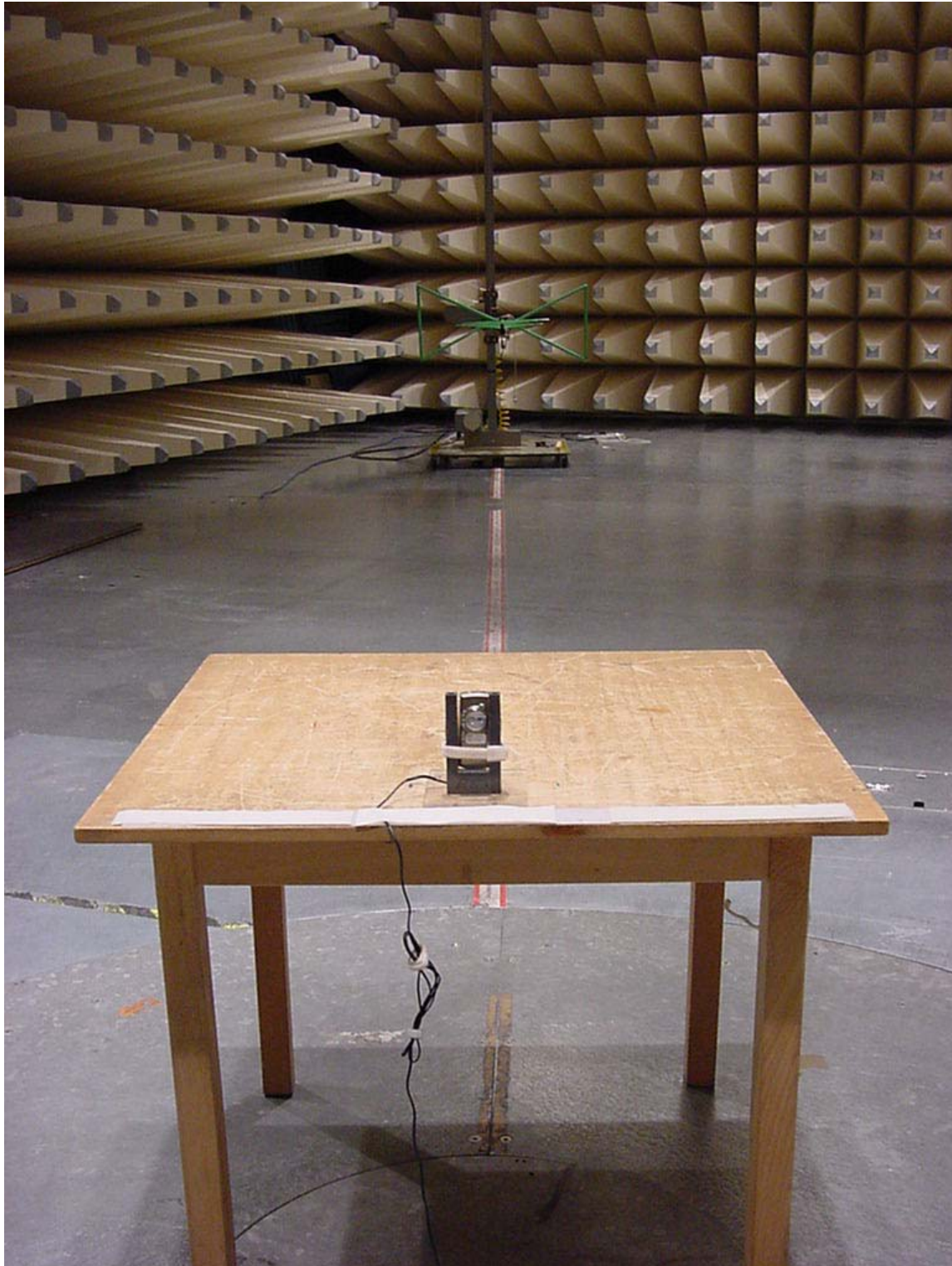
Photo 1: Radiated Emissions
