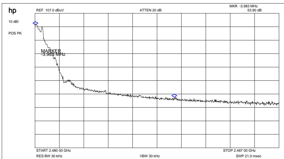
Plot 2: Marker-Delta Method (single carrier)
