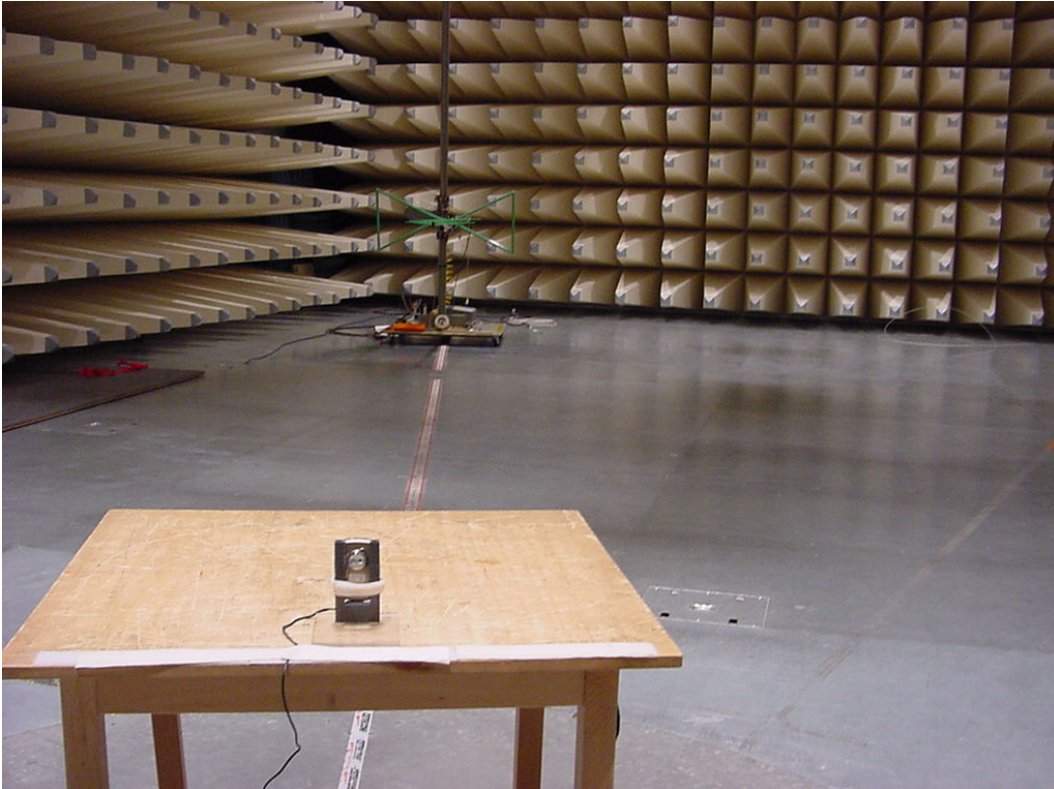
Photo 4 (Radiated Emissions):
