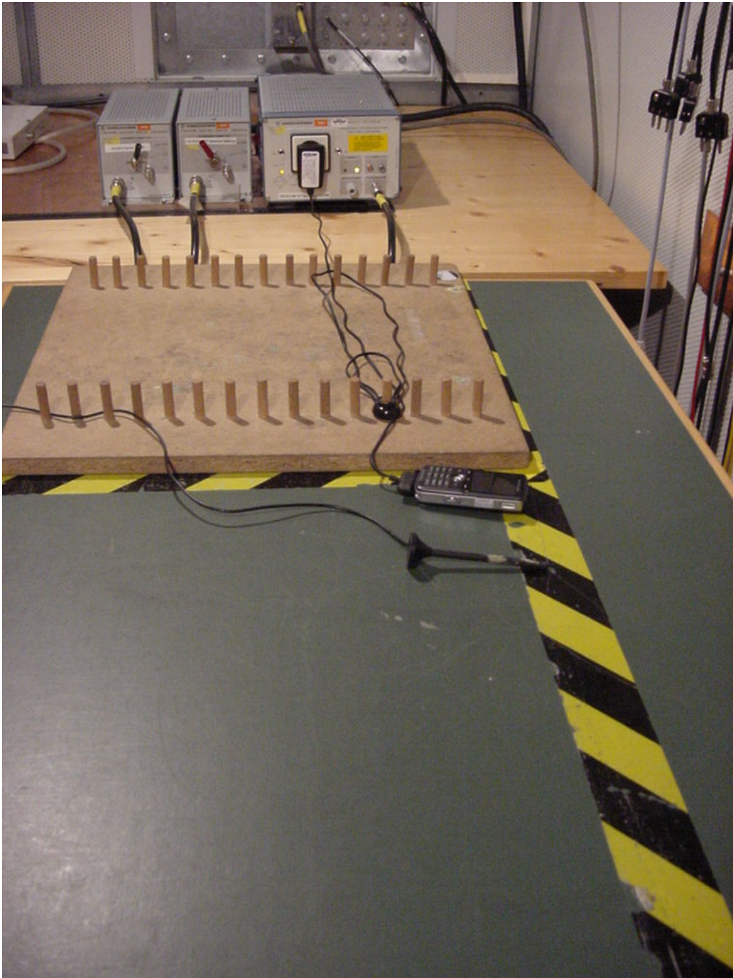
Photo 3 (Conducted Emissions):
