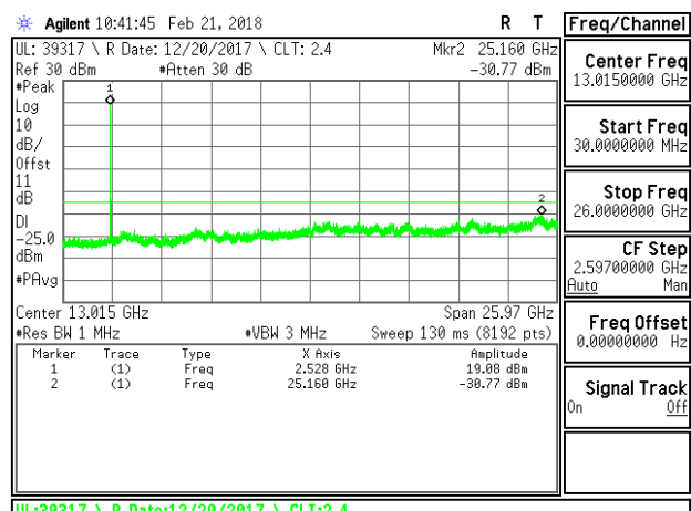
LTE B7 15MHz 16QAM Middle Channel RB1-0
