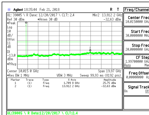
LTE B2 15MHz QPSK Low Channel RB1-0
