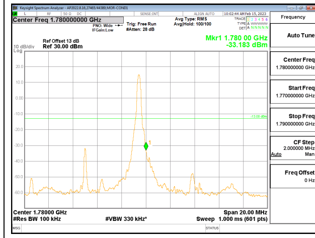
LTE66 10MHz 16QAM HIGH Ch RB1-49
