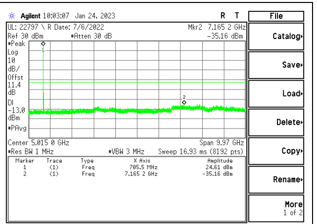
LTE12 3MHz QPSK MID Ch RB1-0
