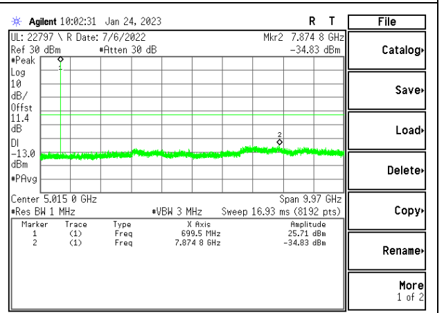
LTE12 3MHz 16QAM LOW Ch RB1-0
