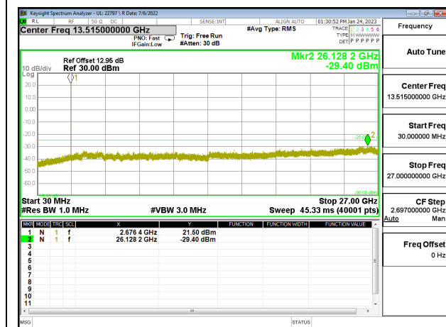
LTE41 15MHz QPSK HIGH Ch RB1-0
