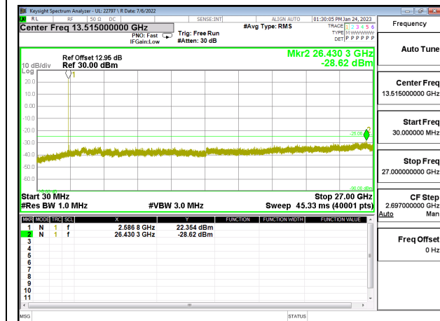
LTE41 15MHz 16QAM MID Ch RB1-0
