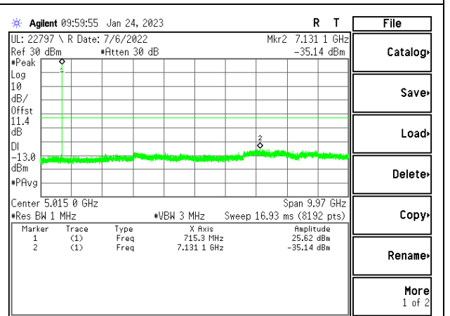
LTE12 1.4MHz 16QAM HIGH Ch RB1-0
