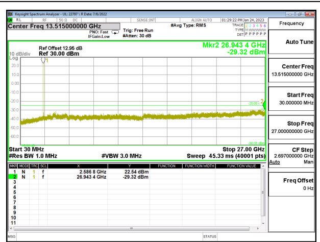
LTE41 15MHz QPSK MID Ch RB1-0
