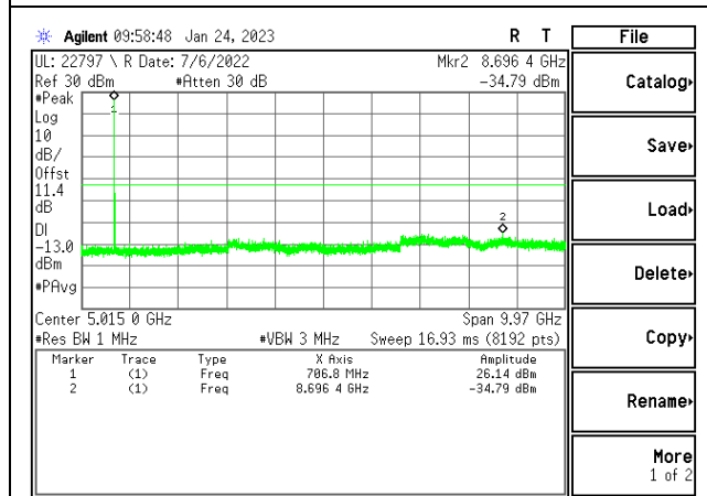
LTE12 1.4MHz 16QAM MID Ch RB1-0
