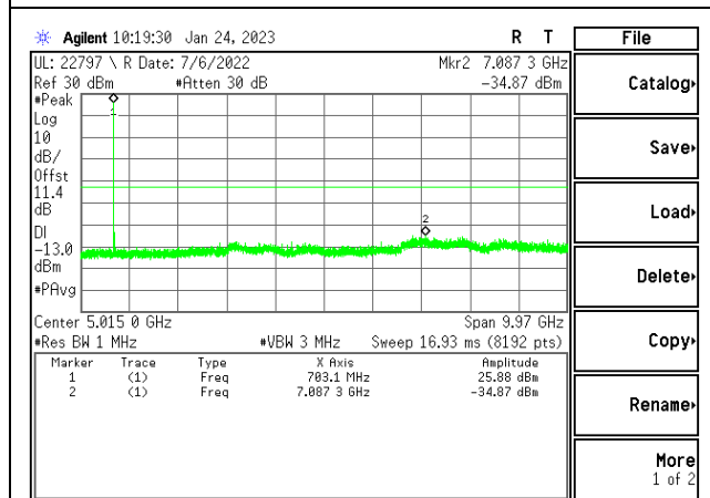
LTE12 10MHz 16QAM MID Ch RB1-0
