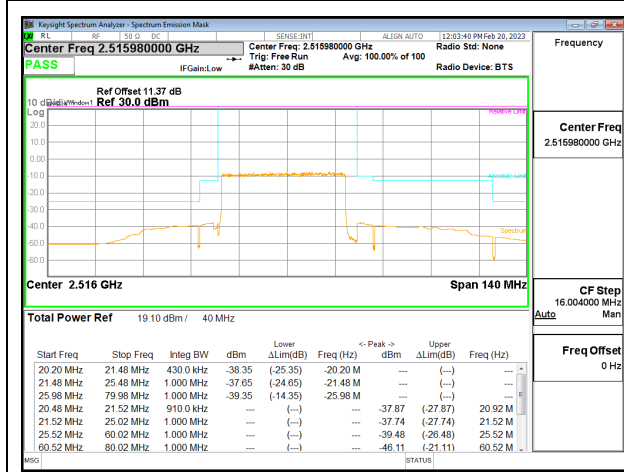
5G NR n41 40MHz 16QAM Low Channel RB100-0
