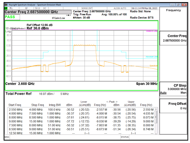
LTE41 5MHz QPSK HIGH Ch RB25-0
