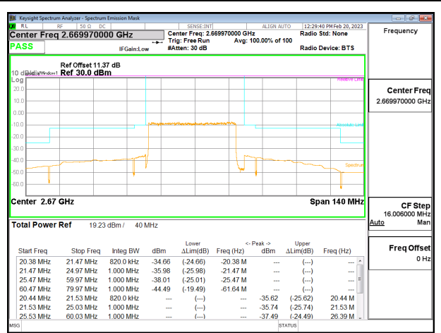
5G NR n41 40MHz 16QAM High Channel RB100-0
