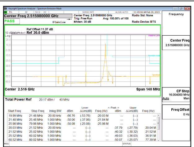
5G NR n41 40MHz BPSK Low Channel RB1-104
