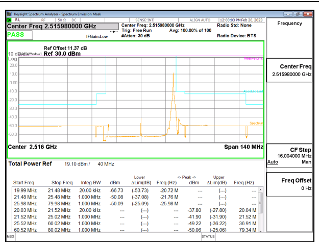
5G NR n41 40MHz 16QAM Low Channel RB1-104
