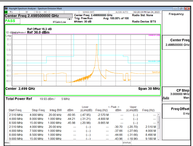
LTE41 5MHz QPSK LOW Ch RB1-24
