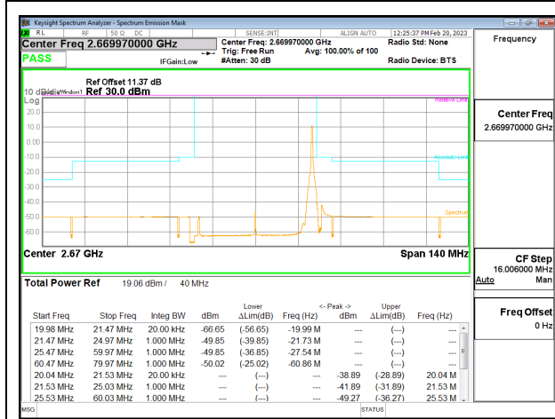
5G NR n41 40MHz 16QAM High Channel RB1-104
