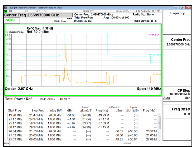
5G NR n41 40MHz 16QAM High Channel RB1-0
