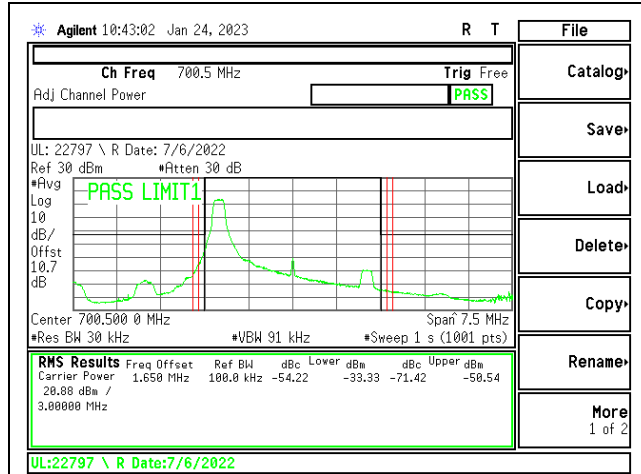
LTE12 3MHz QPSK LOW Ch RB1-0
