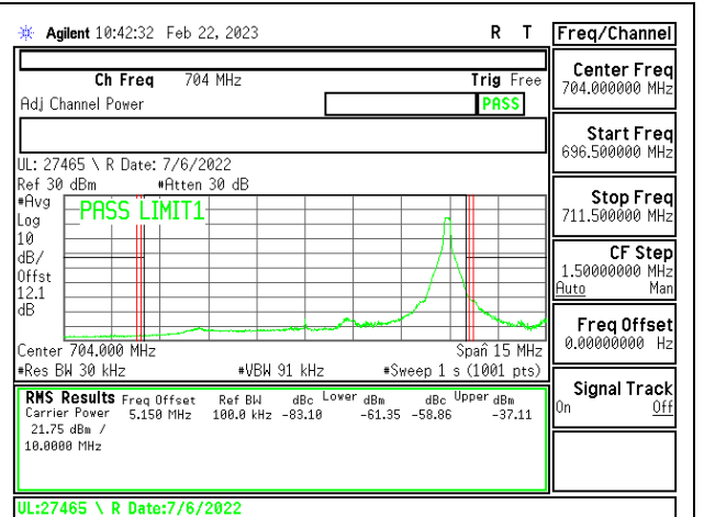
LTE12 10MHz 16QAM LOW Ch RB1-49
