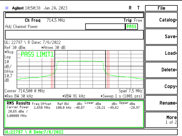
LTE12 3MHz QPSK HIGH Ch RB15-0
