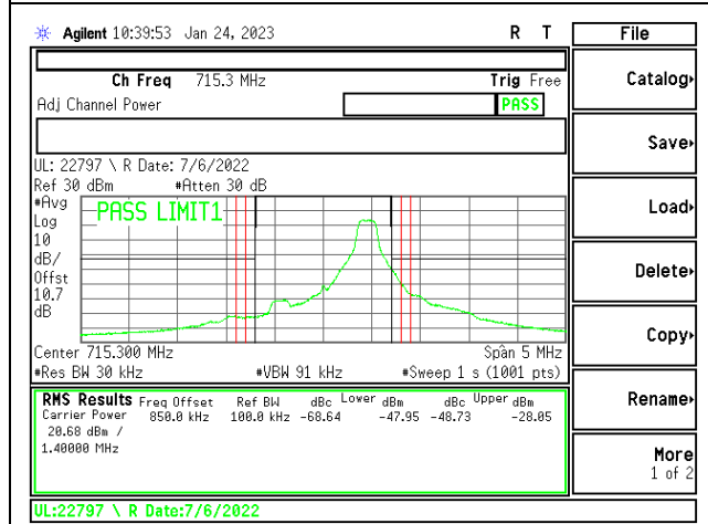
LTE12 1.4MHz QPSK HIGH Ch RB1-5
