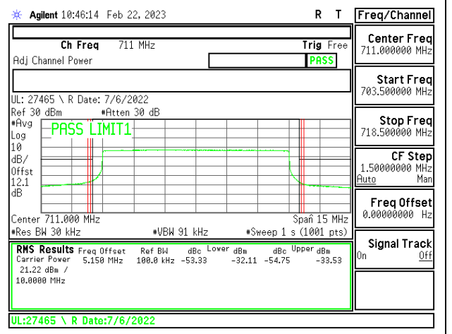
LTE12 10MHz 16QAM HIGH Ch RB50-0
