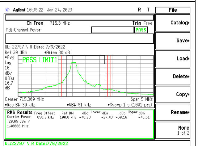
LTE12 1.4MHz QPSK HIGH Ch RB1-0
