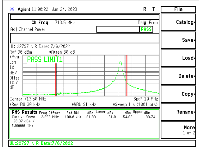
LTE12 5MHz QPSK HIGH Ch RB1-24
