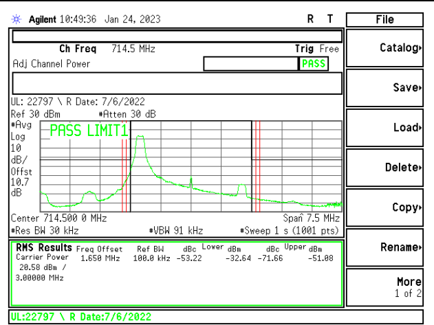
LTE12 3MHz QPSK HIGH Ch RB1-0
