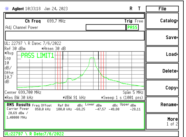
LTE12 1.4MHz QPSK LOW Ch RB1-5
