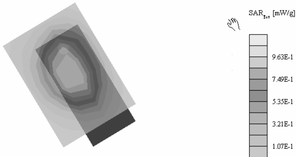
Distributions of max SAR in GSM 850 mode at 824.2MHz. Measured against the head for cheek phone position
