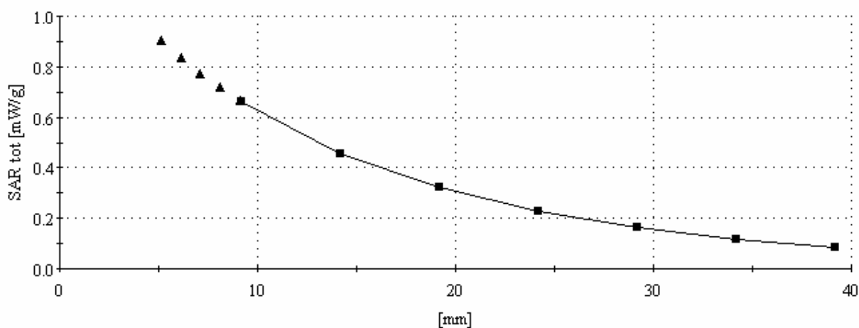
Z(x) distribution of max SAR in GSM 850 mode at 824.2MHz. Measured against the head for cheek phone position
