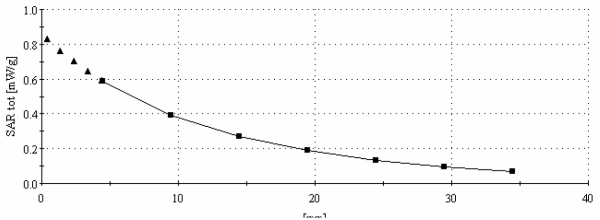
Z(x) distribution of max SAR in GSM 850 mode at 824.2MHz. Measured against the body for back phone position to the phantom
