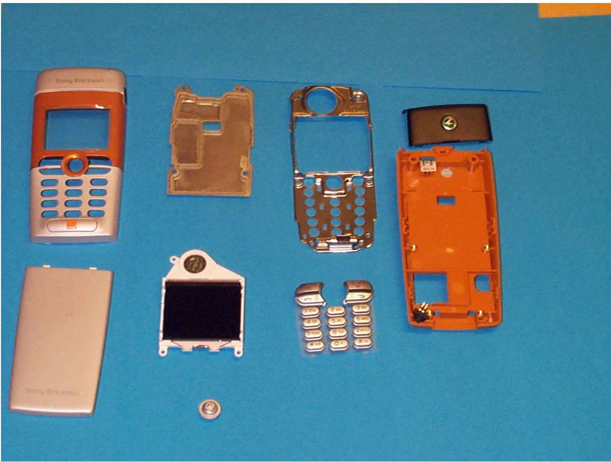
Photograph 5: shielded enclosure of EUT
