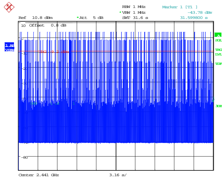
Fig.70. Time of occupancy (Dwell Time): Channel 39, \pi/4 DQPSK -DH5
