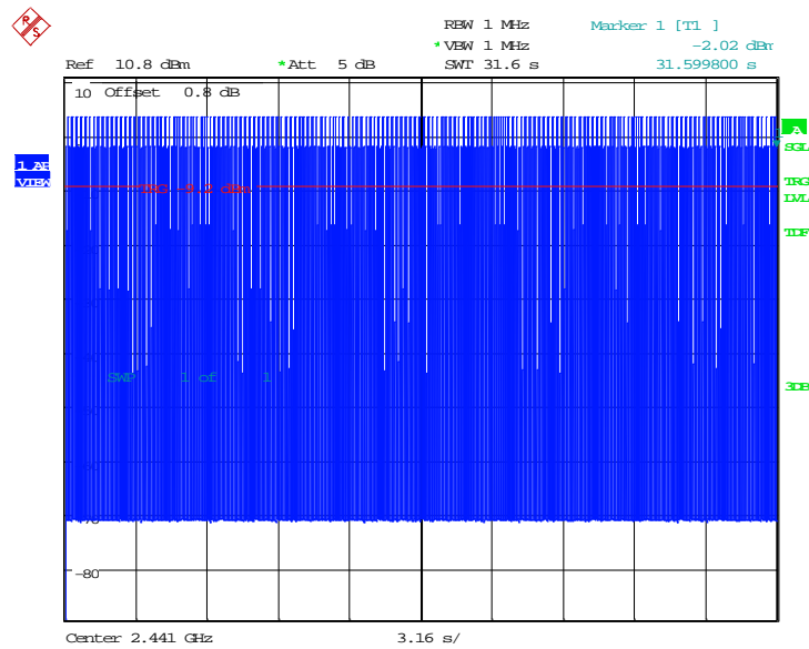
Fig.66. Time of occupancy (Dwell Time): Channel 39, \pi/4 DQPSK -DH1
