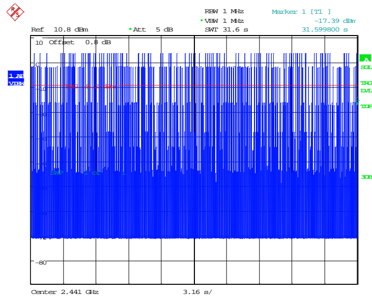
Fig.68. Time of occupancy (Dwell Time): Channel 39, \pi/4 DQPSK -DH3
